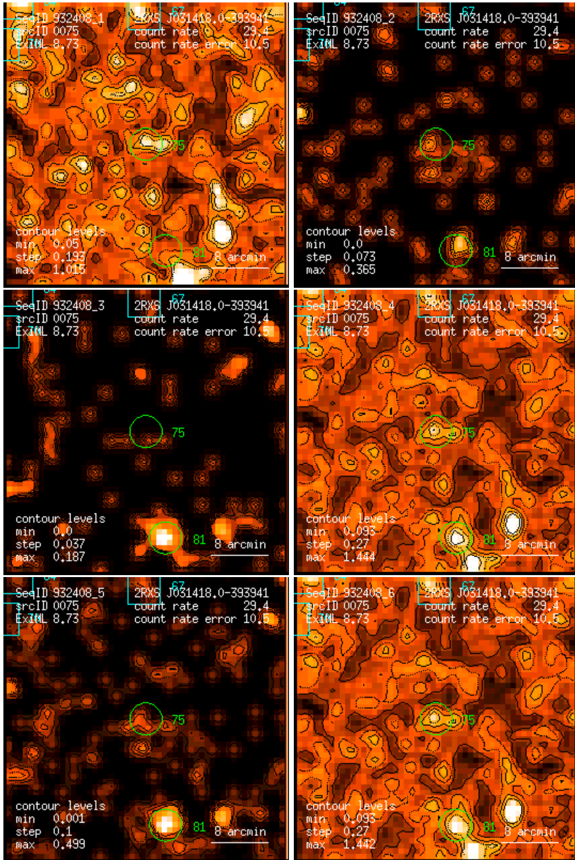
Figure 75: RASS 932408: detection 0075: band rate images, Gaussian filter: (1) PSPC channels 11 – 41, (2) 52 – 90, (3) 91 – 201, (4) 11 – 235, (5) 52 – 201, (6) 11 – 201. Broad band rates in counts/ks. Band rate contour levels in counts/ks/arcmin 2 .
