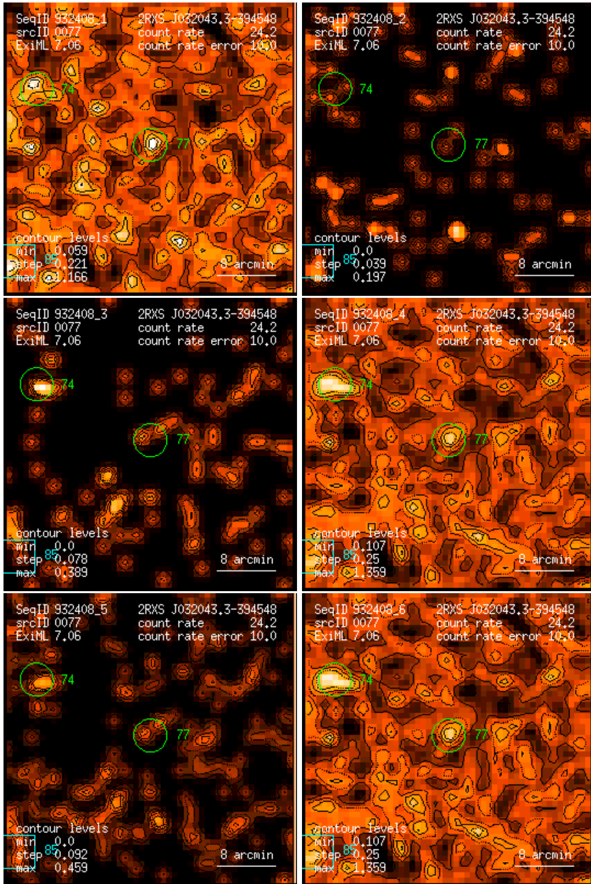
Figure 77: RASS 932408: detection 0077: band rate images, Gaussian filter: (1) PSPC channels 11 – 41, (2) 52 – 90, (3) 91 – 201, (4) 11 – 235, (5) 52 – 201, (6) 11 – 201. Broad band rates in counts/ks. Band rate contour levels in counts/ks/arcmin 2 .
