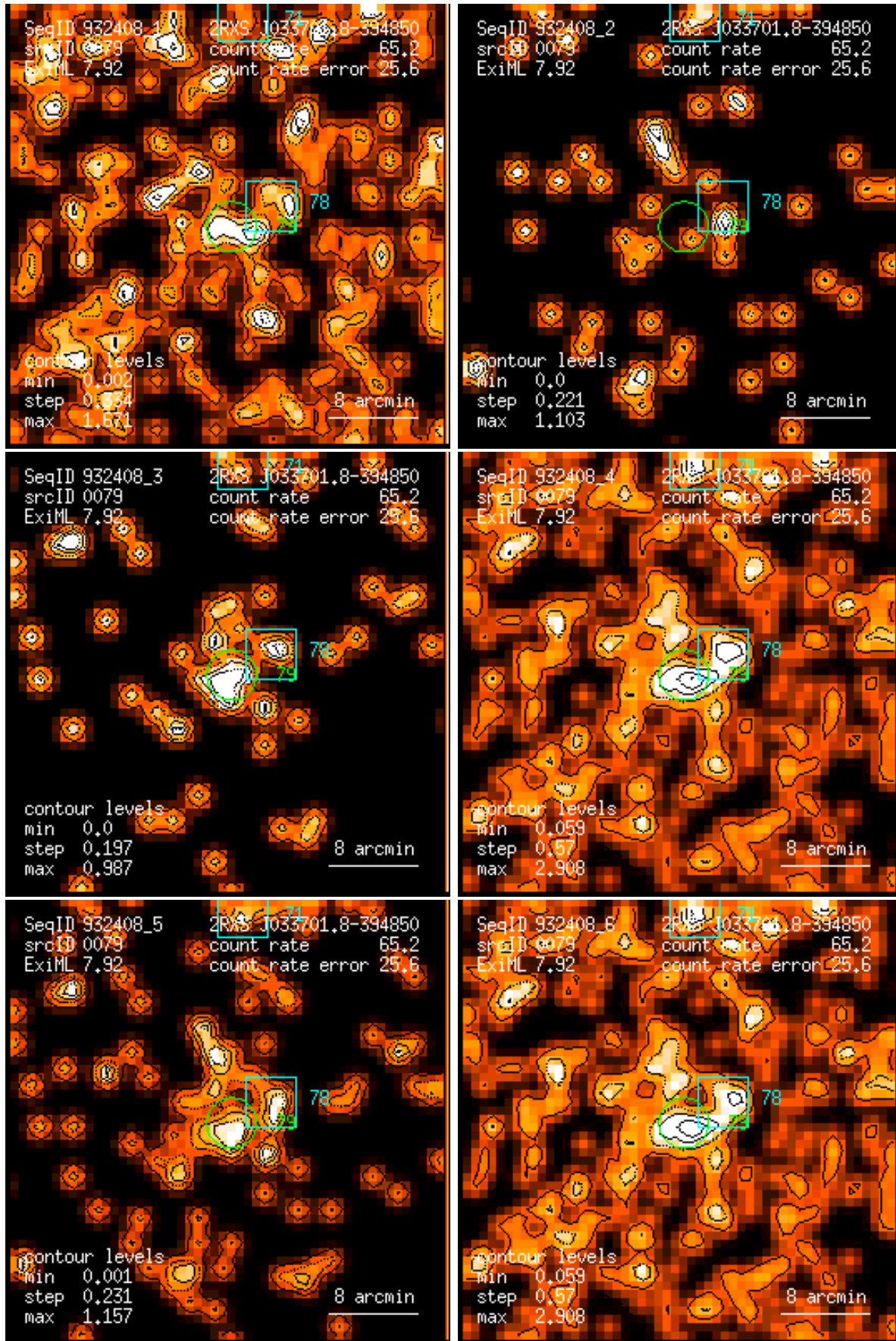
Figure 79: RASS 932408: detection 0079: band rate images, Gaussian filter: (1) PSPC channels 11 – 41, (2) 52 – 90, (3) 91 – 201, (4) 11 – 235, (5) 52 – 201, (6) 11 – 201. Broad band rates in counts/ks. Band rate contour levels in counts/ks/arcmin 2 .
