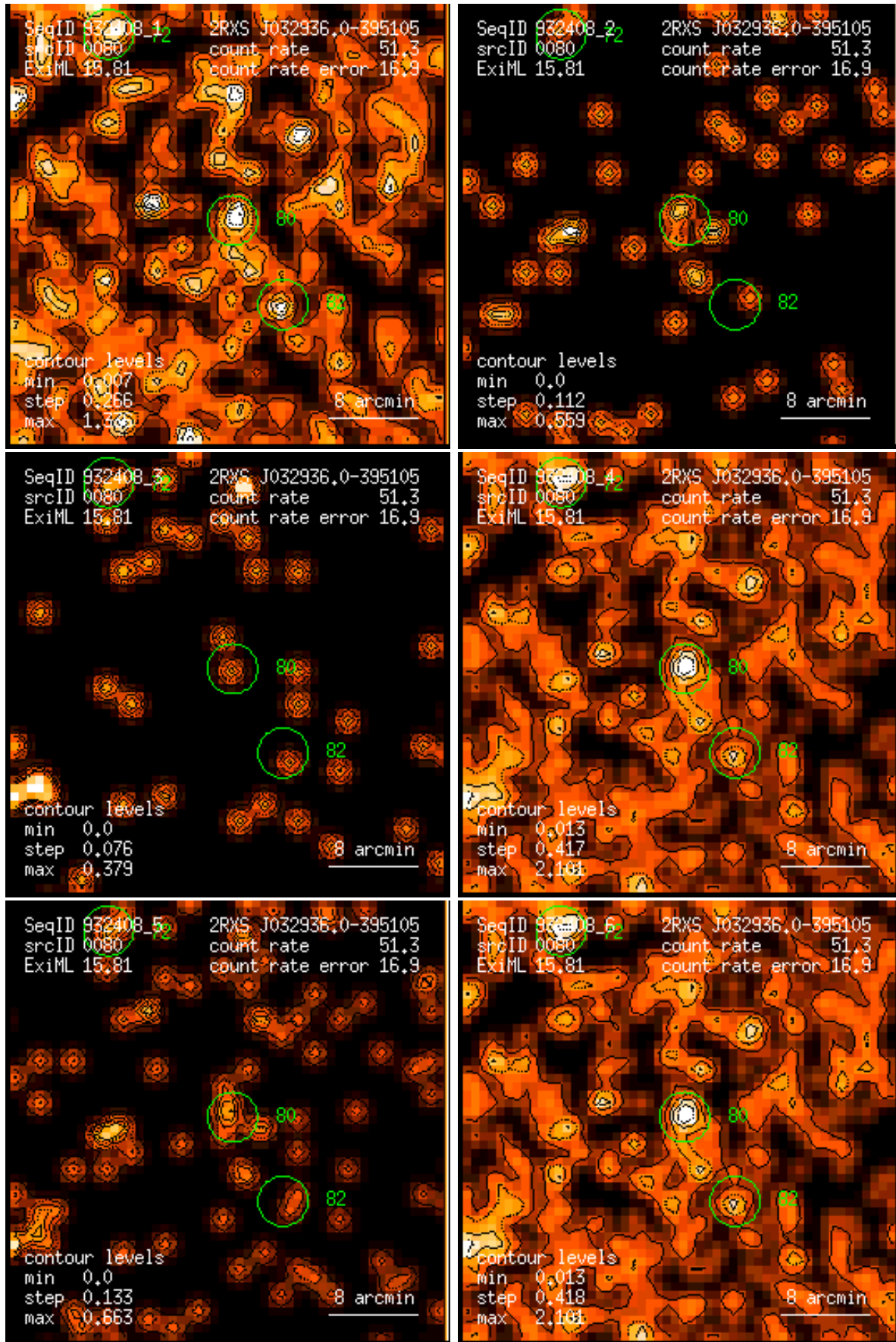
Figure 80: RASS 932408: detection 0080: band rate images, Gaussian filter: (1) PSPC channels 11 – 41, (2) 52 – 90, (3) 91 – 201, (4) 11 – 235, (5) 52 – 201, (6) 11 – 201. Broad band rates in counts/ks. Band rate contour levels in counts/ks/arcmin 2 .
