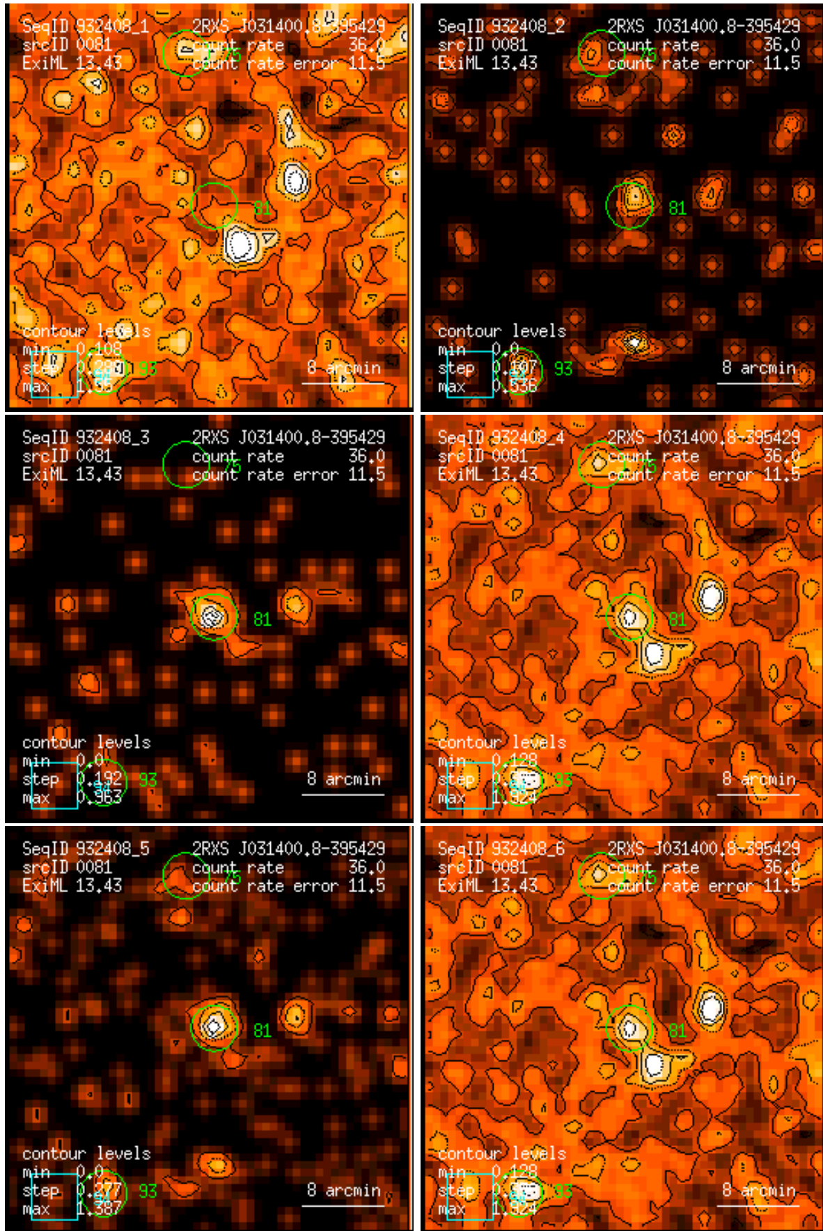
Figure 81: RASS 932408: detection 0081: band rate images, Gaussian filter: (1) PSPC channels 11 – 41, (2) 52 – 90, (3) 91 – 201, (4) 11 – 235, (5) 52 – 201, (6) 11 – 201. Broad band rates in counts/ks. Band rate contour levels in counts/ks/arcmin 2 .
