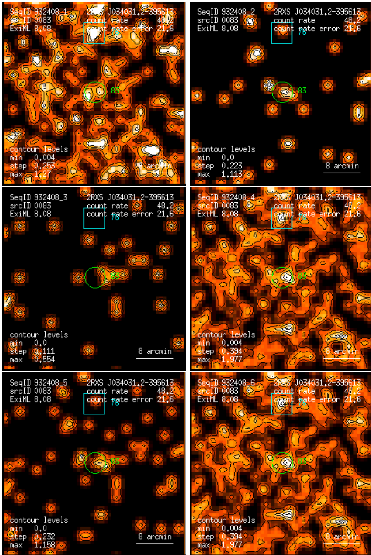
Figure 83: RASS 932408: detection 0083: band rate images, Gaussian filter: (1) PSPC channels 11 – 41, (2) 52 – 90, (3) 91 – 201, (4) 11 – 235, (5) 52 – 201, (6) 11 – 201. Broad band rates in counts/ks. Band rate contour levels in counts/ks/arcmin 2 .
