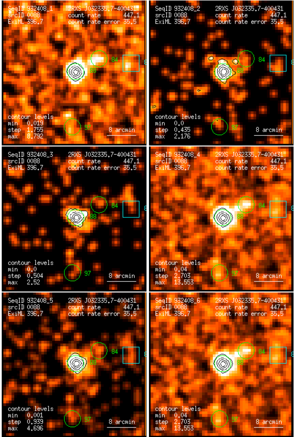
Figure 88: RASS 932408: detection 0088: band rate images, Gaussian filter: (1) PSPC channels 11 – 41, (2) 52 – 90, (3) 91 – 201, (4) 11 – 235, (5) 52 – 201, (6) 11 – 201. Broad band rates in counts/ks. Band rate contour levels in counts/ks/arcmin 2 .
