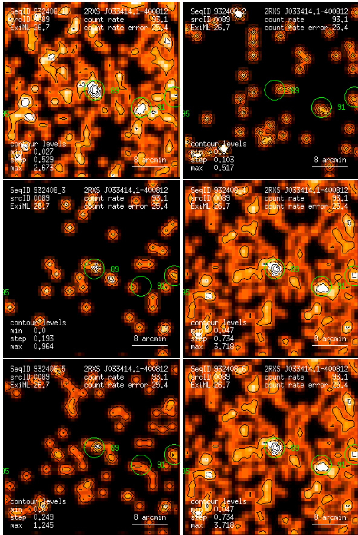
Figure 89: RASS 932408: detection 0089: band rate images, Gaussian filter: (1) PSPC channels 11 – 41, (2) 52 – 90, (3) 91 – 201, (4) 11 – 235, (5) 52 – 201, (6) 11 – 201. Broad band rates in counts/ks. Band rate contour levels in counts/ks/arcmin 2 .
