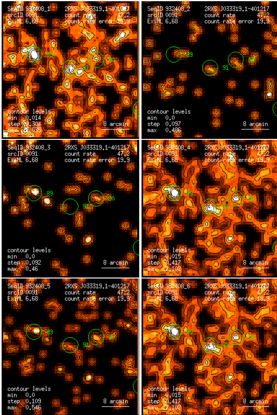
Figure 91: RASS 932408: detection 0091: band rate images, Gaussian filter: (1) PSPC channels 11 – 41, (2) 52 – 90, (3) 91 – 201, (4) 11 – 235, (5) 52 – 201, (6) 11 – 201. Broad band rates in counts/ks. Band rate contour levels in counts/ks/arcmin 2 .
