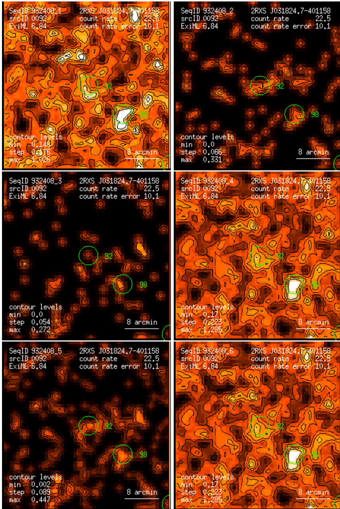
Figure 92: RASS 932408: detection 0092: band rate images, Gaussian filter: (1) PSPC channels 11 – 41, (2) 52 – 90, (3) 91 – 201, (4) 11 – 235, (5) 52 – 201, (6) 11 – 201. Broad band rates in counts/ks. Band rate contour levels in counts/ks/arcmin 2 .
