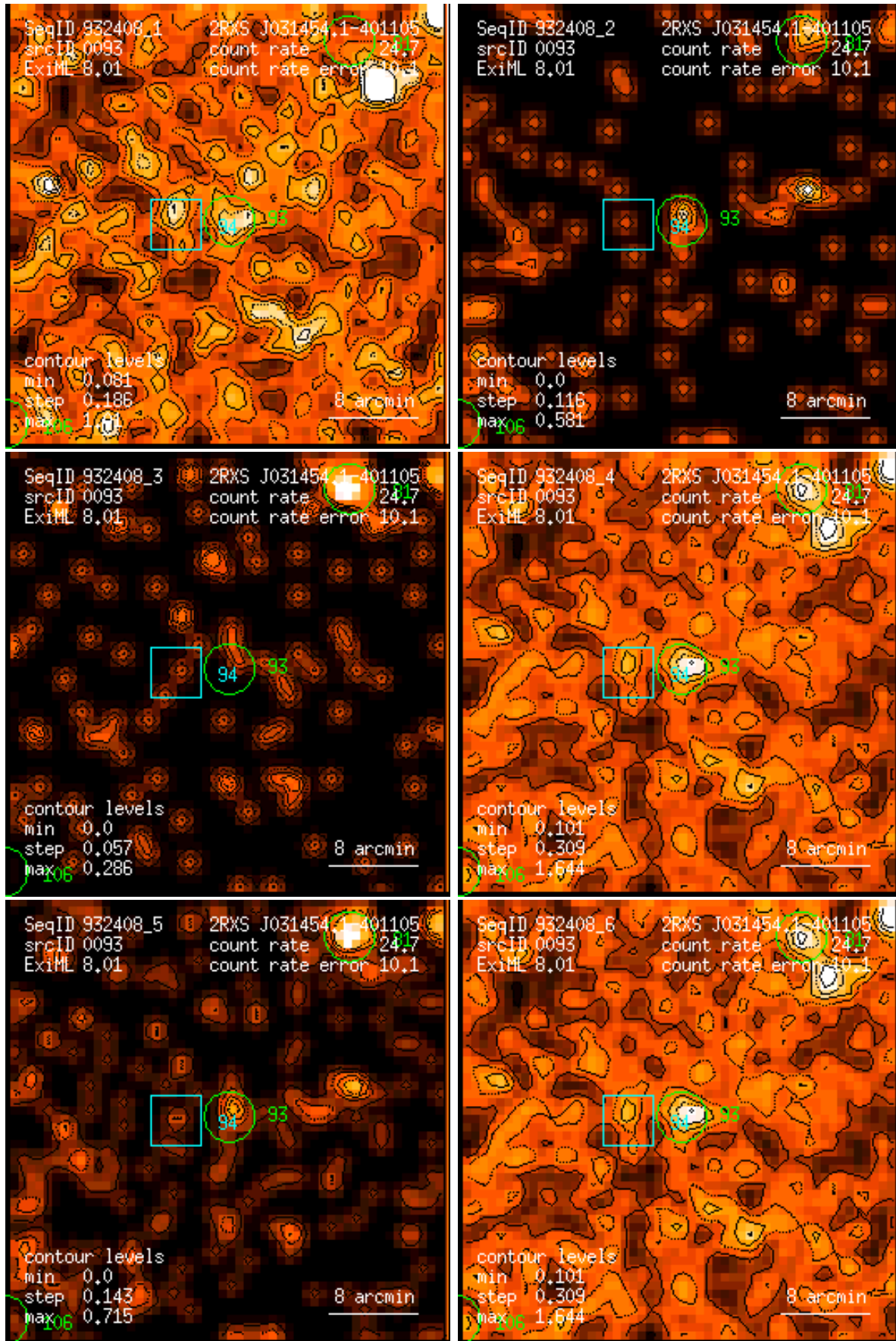
Figure 93: RASS 932408: detection 0093: band rate images, Gaussian filter: (1) PSPC channels 11 – 41, (2) 52 – 90, (3) 91 – 201, (4) 11 – 235, (5) 52 – 201, (6) 11 – 201. Broad band rates in counts/ks. Band rate contour levels in counts/ks/arcmin 2 .
