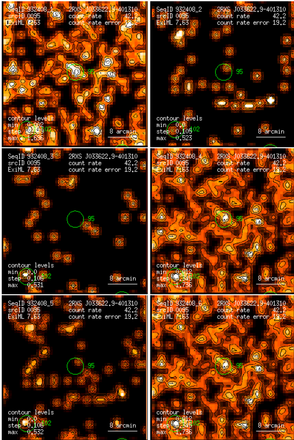
Figure 95: RASS 932408: detection 0095: band rate images, Gaussian filter: (1) PSPC channels 11 – 41, (2) 52 – 90, (3) 91 – 201, (4) 11 – 235, (5) 52 – 201, (6) 11 – 201. Broad band rates in counts/ks. Band rate contour levels in counts/ks/arcmin 2 .
