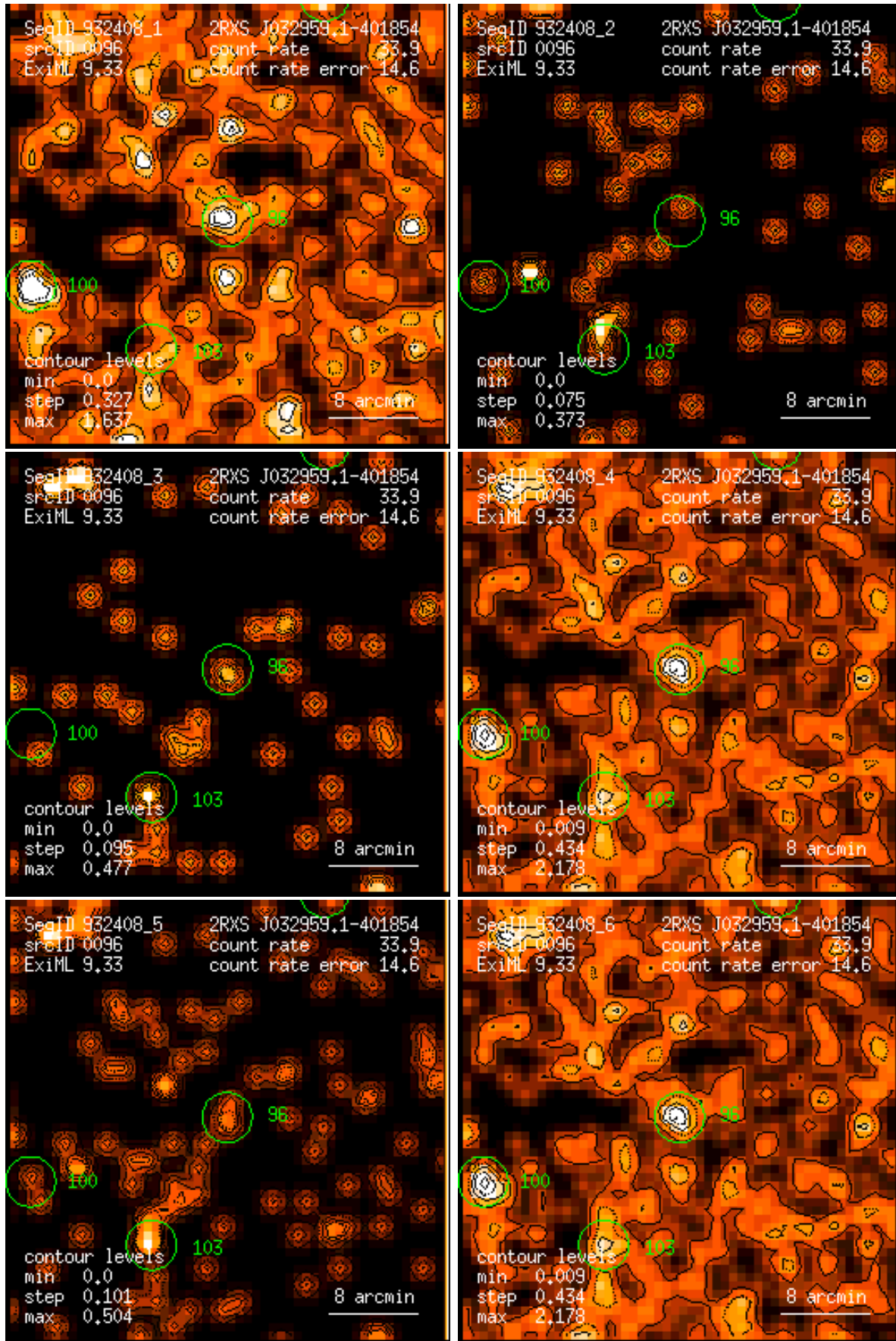
Figure 96: RASS 932408: detection 0096: band rate images, Gaussian filter: (1) PSPC channels 11 – 41, (2) 52 – 90, (3) 91 – 201, (4) 11 – 235, (5) 52 – 201, (6) 11 – 201. Broad band rates in counts/ks. Band rate contour levels in counts/ks/arcmin 2 .
