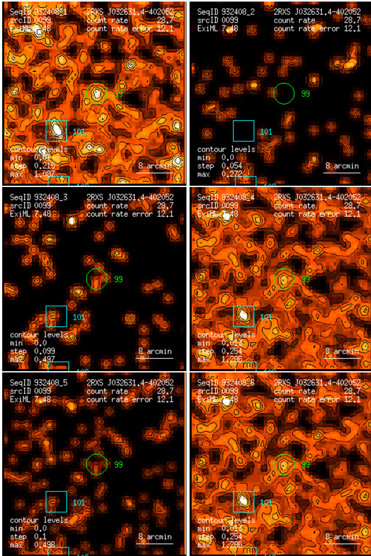
Figure 99: RASS 932408: detection 0099: band rate images, Gaussian filter: (1) PSPC channels 11 – 41, (2) 52 – 90, (3) 91 – 201, (4) 11 – 235, (5) 52 – 201, (6) 11 – 201. Broad band rates in counts/ks. Band rate contour levels in counts/ks/arcmin 2 .
