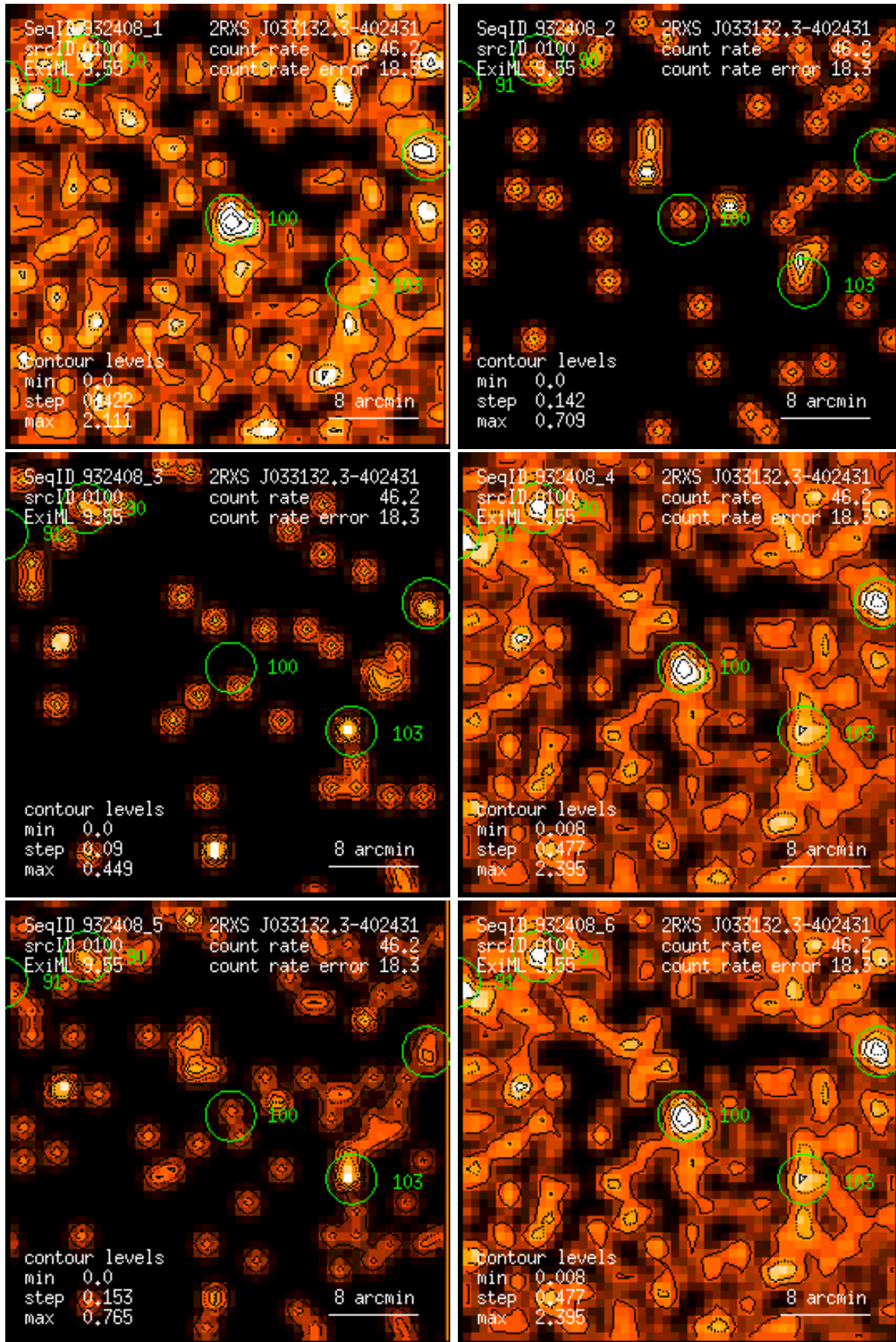
Figure 100: RASS 932408: detection 0100: band rate images, Gaussian filter: (1) PSPC channels 11 – 41, (2) 52 – 90, (3) 91 – 201, (4) 11 – 235, (5) 52 – 201, (6) 11 – 201. Broad band rates in counts/ks. Band rate contour levels in counts/ks/arcmin 2 .
