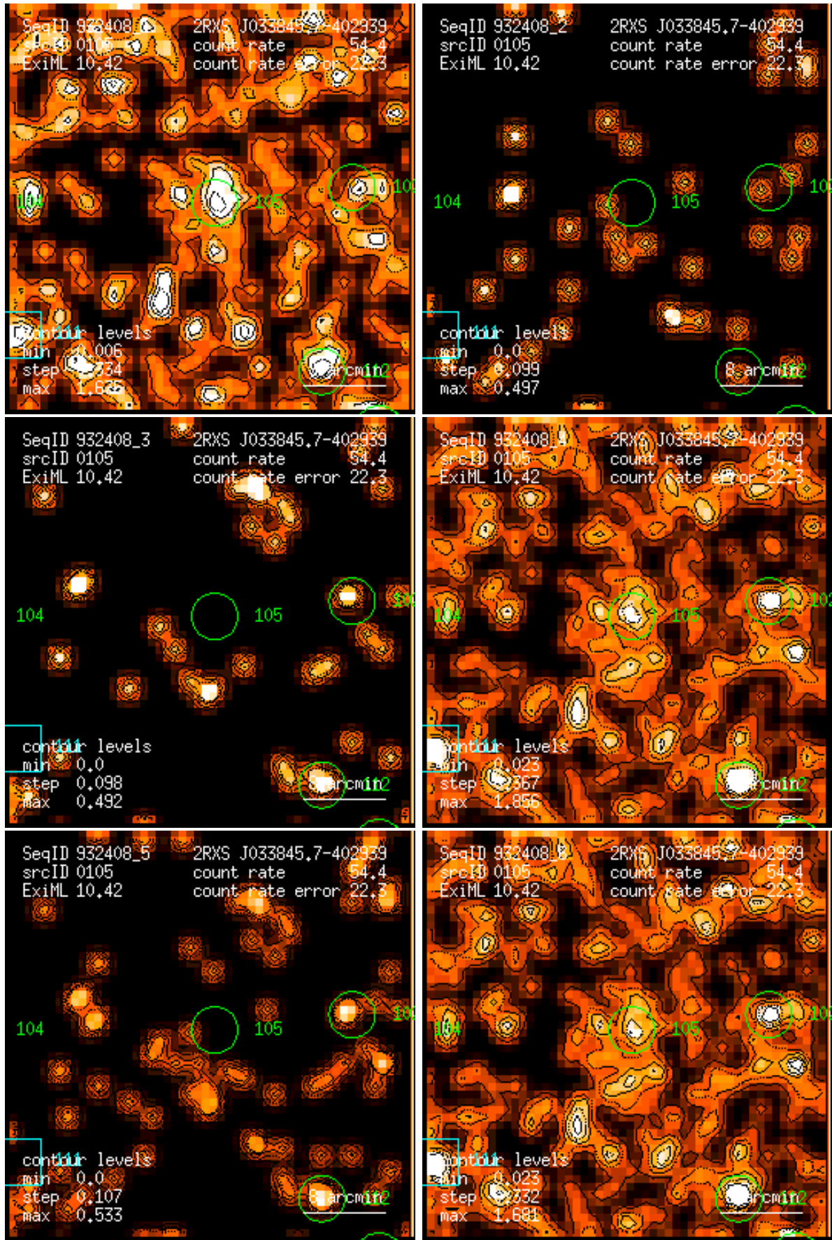
Figure 105: RASS 932408: detection 0105: band rate images, Gaussian filter: (1) PSPC channels 11 – 41, (2) 52 – 90, (3) 91 – 201, (4) 11 – 235, (5) 52 – 201, (6) 11 – 201. Broad band rates in counts/ks. Band rate contour levels in counts/ks/arcmin 2 .
