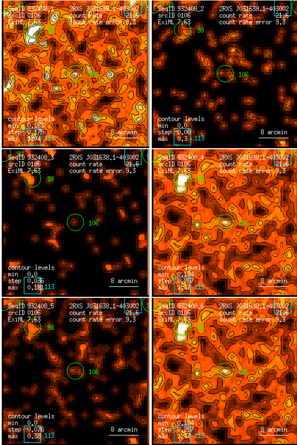
Figure 106: RASS 932408: detection 0106: band rate images, Gaussian filter: (1) PSPC channels 11 – 41, (2) 52 – 90, (3) 91 – 201, (4) 11 – 235, (5) 52 – 201, (6) 11 – 201. Broad band rates in counts/ks. Band rate contour levels in counts/ks/arcmin 2 .
