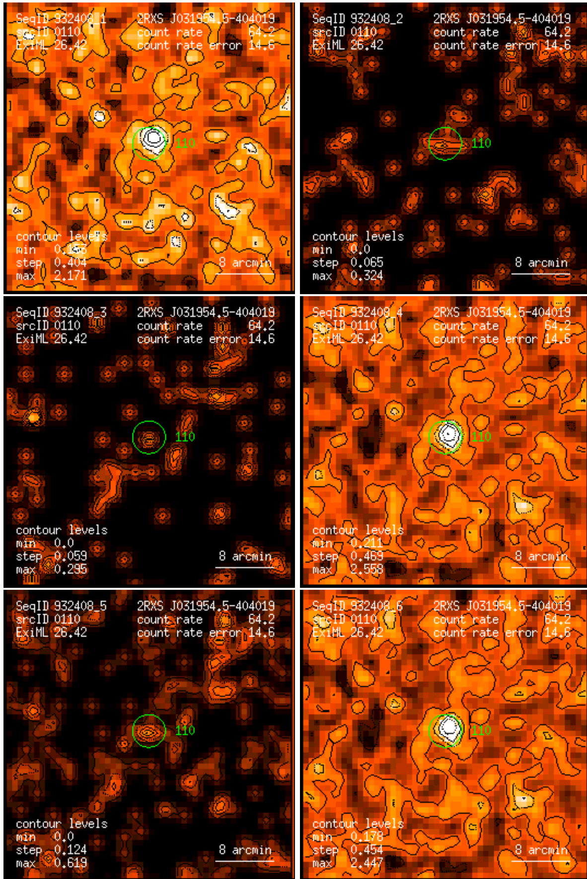
Figure 110: RASS 932408: detection 0110: band rate images, Gaussian filter: (1) PSPC channels 11 – 41, (2) 52 – 90, (3) 91 – 201, (4) 11 – 235, (5) 52 – 201, (6) 11 – 201. Broad band rates in counts/ks. Band rate contour levels in counts/ks/arcmin 2 .
