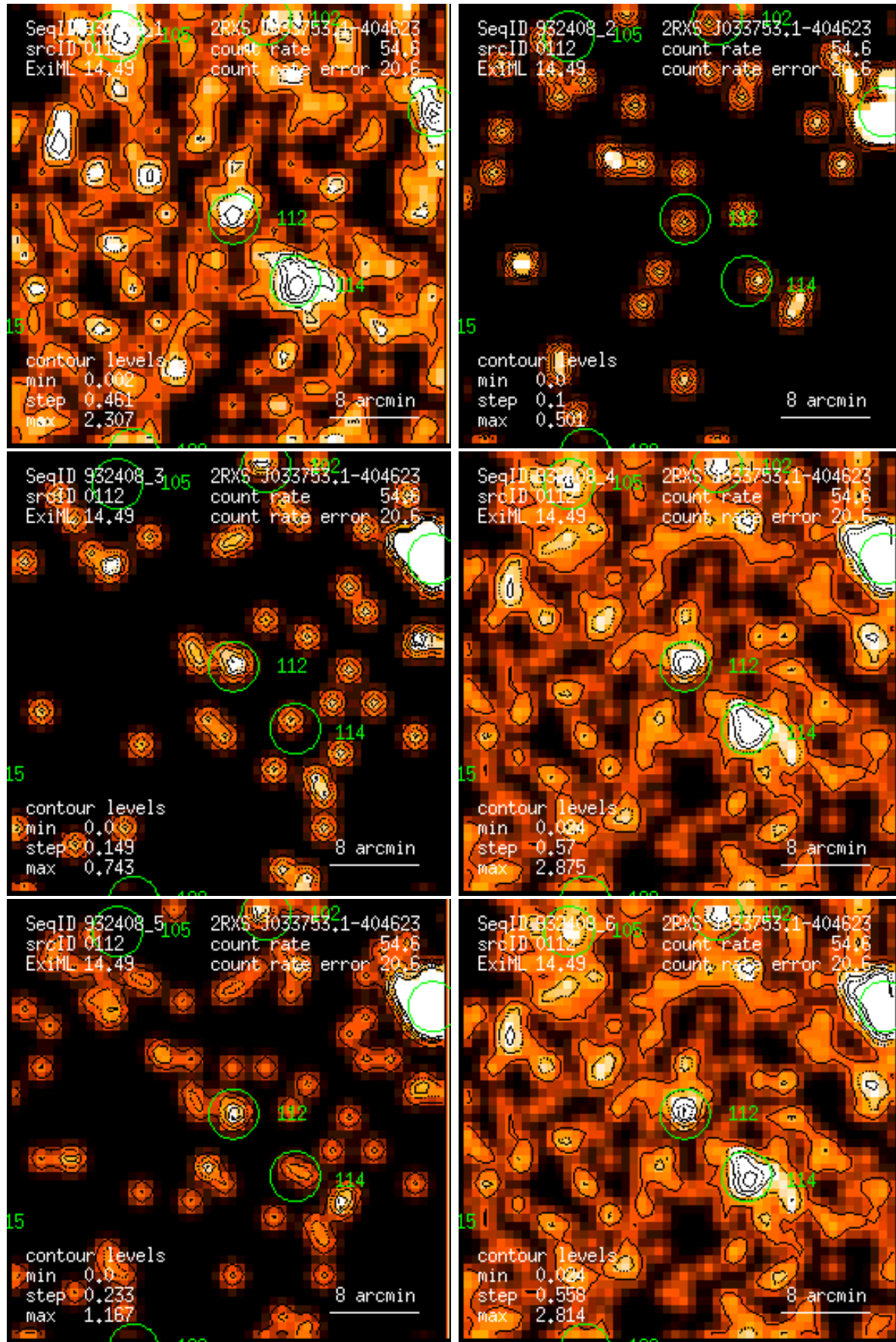
Figure 112: RASS 932408: detection 0112: band rate images, Gaussian filter: (1) PSPC channels 11 – 41, (2) 52 – 90, (3) 91 – 201, (4) 11 – 235, (5) 52 – 201, (6) 11 – 201. Broad band rates in counts/ks. Band rate contour levels in counts/ks/arcmin 2 .
