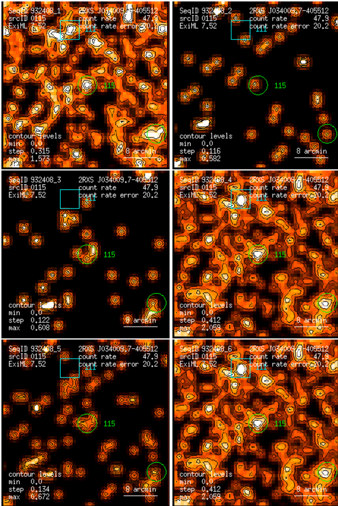
Figure 115: RASS 932408: detection 0115: band rate images, Gaussian filter: (1) PSPC channels 11 – 41, (2) 52 – 90, (3) 91 – 201, (4) 11 – 235, (5) 52 – 201, (6) 11 – 201. Broad band rates in counts/ks. Band rate contour levels in counts/ks/arcmin 2 .
