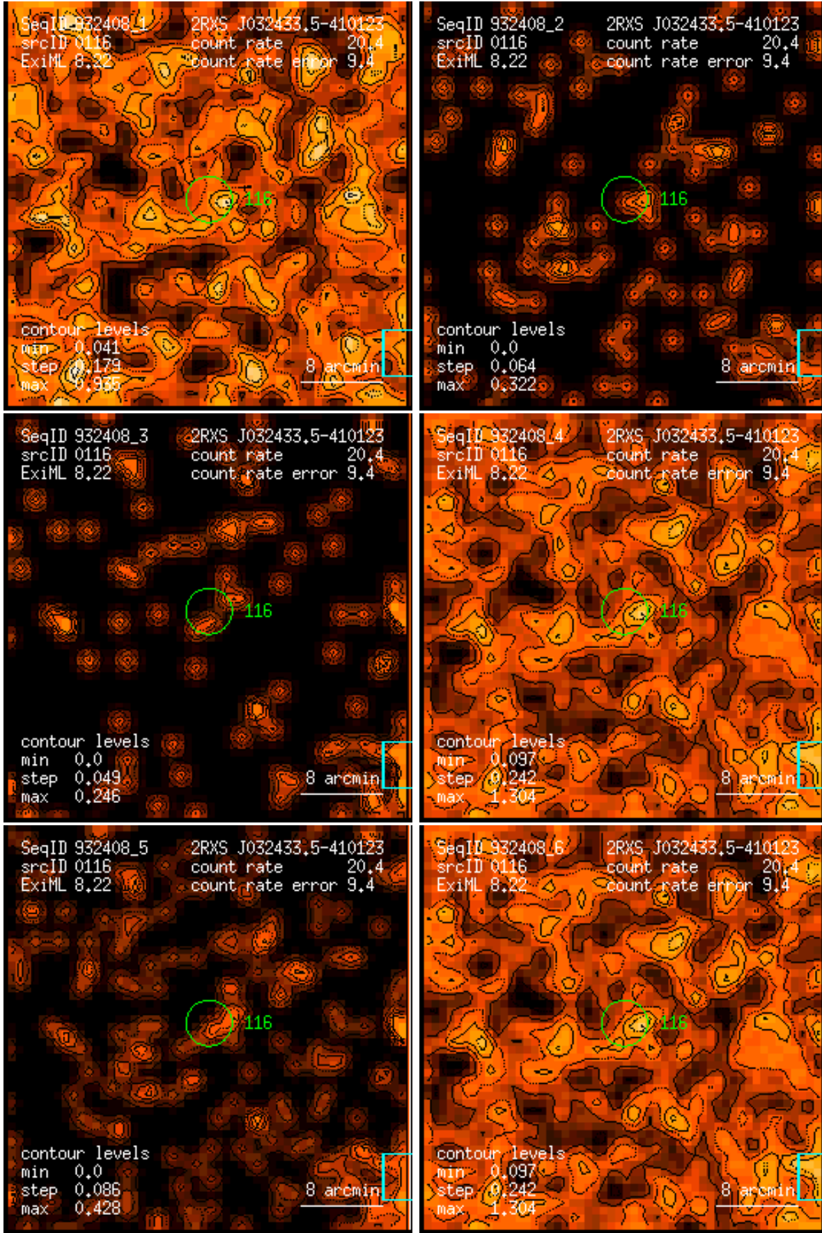
Figure 116: RASS 932408: detection 0116: band rate images, Gaussian filter: (1) PSPC channels 11 – 41, (2) 52 – 90, (3) 91 – 201, (4) 11 – 235, (5) 52 – 201, (6) 11 – 201. Broad band rates in counts/ks. Band rate contour levels in counts/ks/arcmin 2 .
