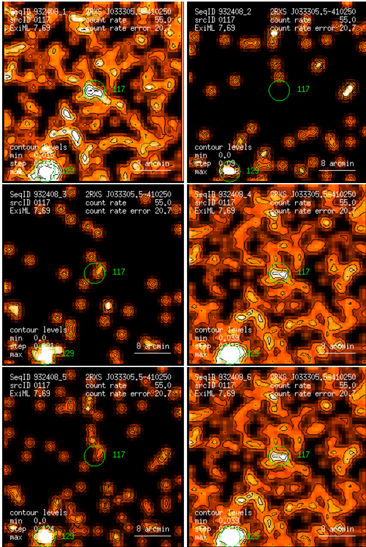
Figure 117: RASS 932408: detection 0117: band rate images, Gaussian filter: (1) PSPC channels 11 – 41, (2) 52 – 90, (3) 91 – 201, (4) 11 – 235, (5) 52 – 201, (6) 11 – 201. Broad band rates in counts/ks. Band rate contour levels in counts/ks/arcmin 2 .
