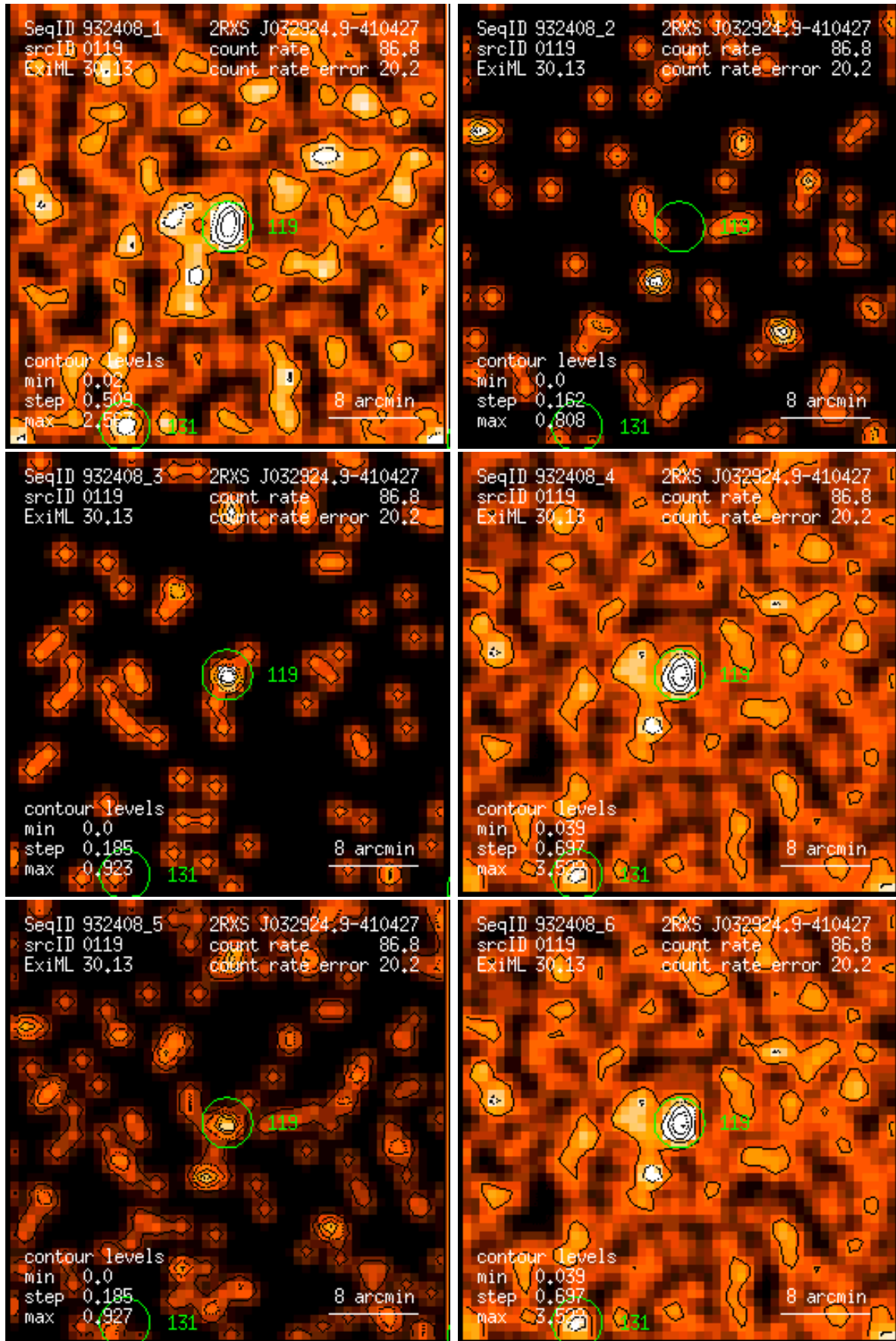
Figure 119: RASS 932408: detection 0119: band rate images, Gaussian filter: (1) PSPC channels 11 – 41, (2) 52 – 90, (3) 91 – 201, (4) 11 – 235, (5) 52 – 201, (6) 11 – 201. Broad band rates in counts/ks. Band rate contour levels in counts/ks/arcmin 2 .
