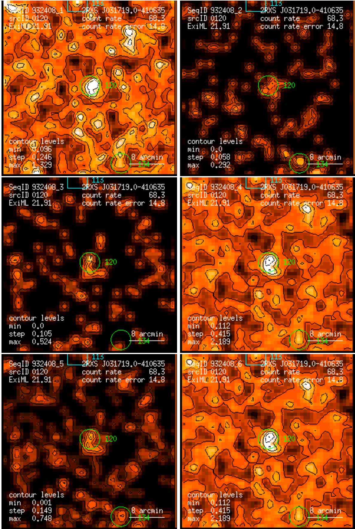
Figure 120: RASS 932408: detection 0120: band rate images, Gaussian filter: (1) PSPC channels 11 – 41, (2) 52 – 90, (3) 91 – 201, (4) 11 – 235, (5) 52 – 201, (6) 11 – 201. Broad band rates in counts/ks. Band rate contour levels in counts/ks/arcmin 2 .
