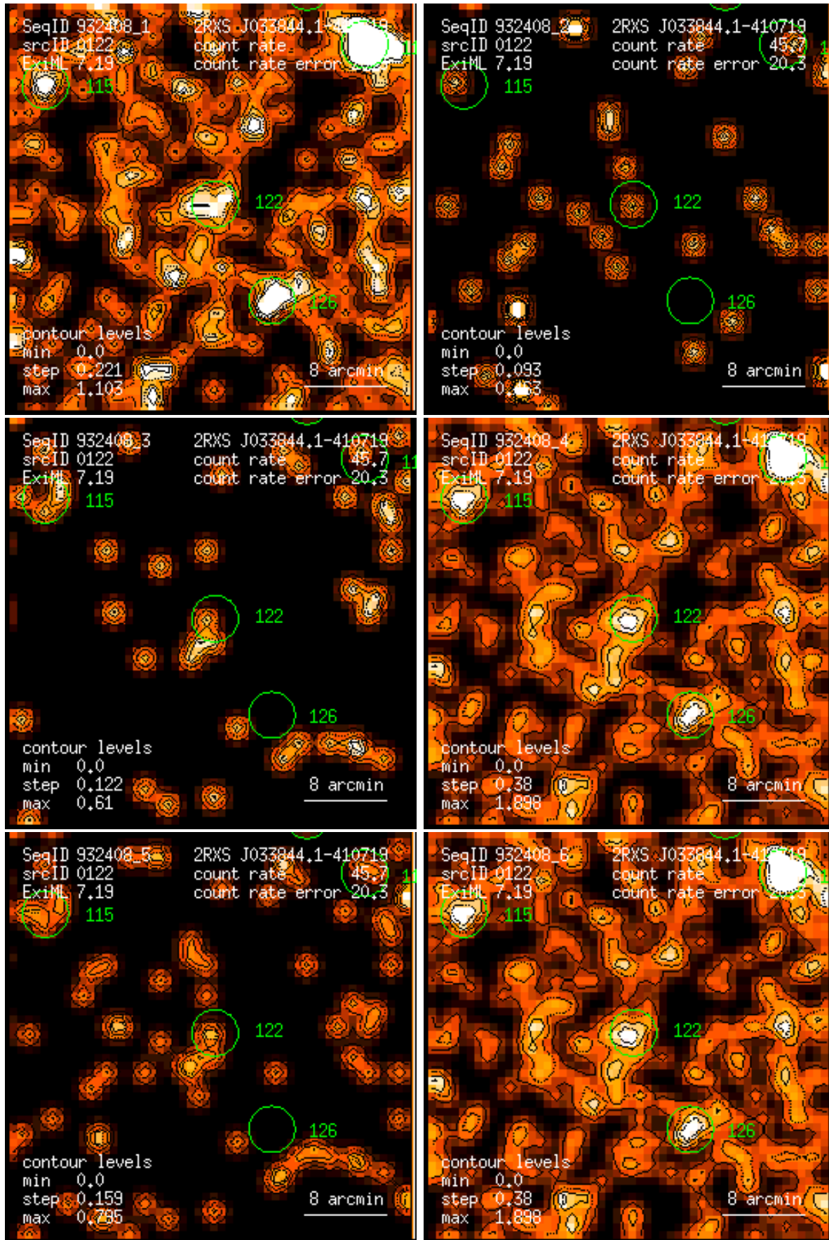
Figure 122: RASS 932408: detection 0122: band rate images, Gaussian filter: (1) PSPC channels 11 – 41, (2) 52 – 90, (3) 91 – 201, (4) 11 – 235, (5) 52 – 201, (6) 11 – 201. Broad band rates in counts/ks. Band rate contour levels in counts/ks/arcmin 2 .
