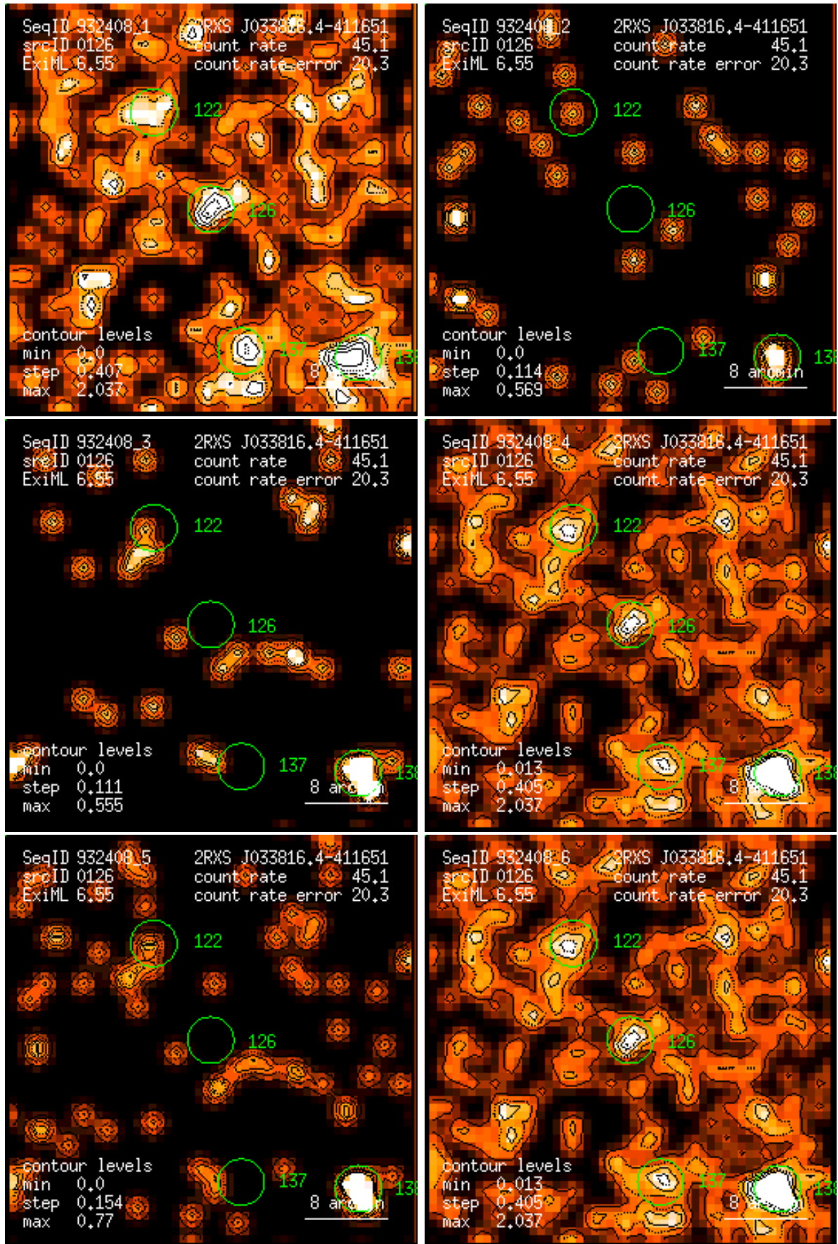
Figure 126: RASS 932408: detection 0126: band rate images, Gaussian filter: (1) PSPC channels 11 – 41, (2) 52 – 90, (3) 91 – 201, (4) 11 – 235, (5) 52 – 201, (6) 11 – 201. Broad band rates in counts/ks. Band rate contour levels in counts/ks/arcmin 2 .
