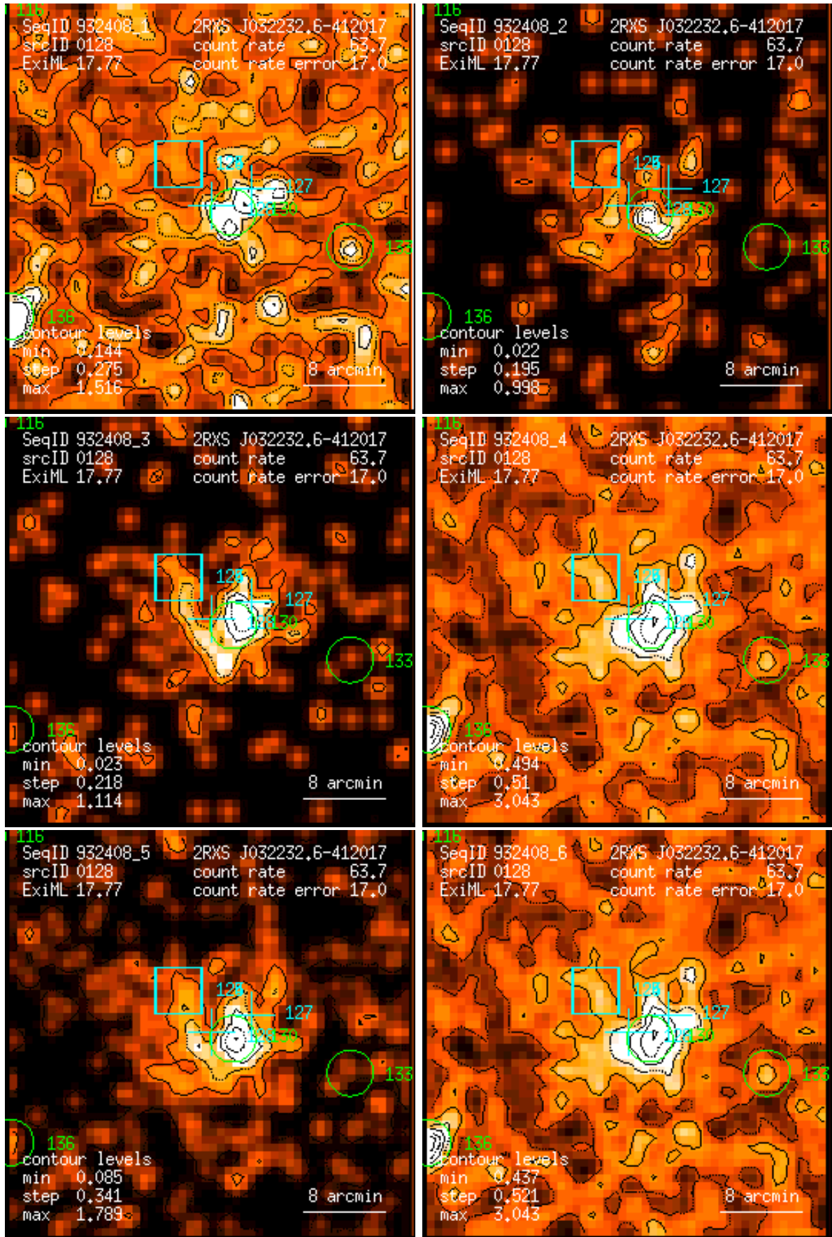
Figure 128: RASS 932408: detection 0128: band rate images, Gaussian filter: (1) PSPC channels 11 – 41, (2) 52 – 90, (3) 91 – 201, (4) 11 – 235, (5) 52 – 201, (6) 11 – 201. Broad band rates in counts/ks. Band rate contour levels in counts/ks/arcmin 2 .
