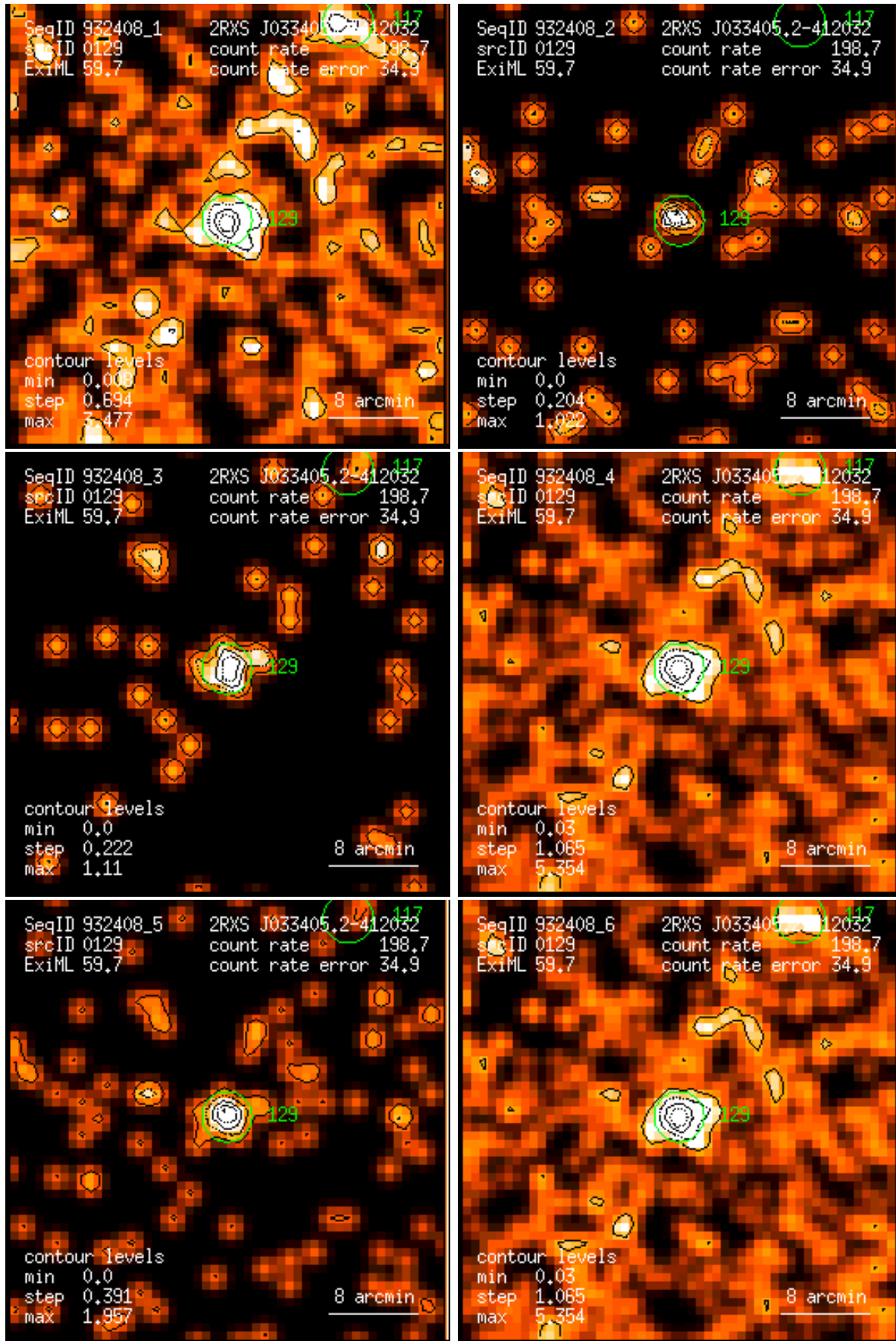
Figure 129: RASS 932408: detection 0129: band rate images, Gaussian filter: (1) PSPC channels 11 – 41, (2) 52 – 90, (3) 91 – 201, (4) 11 – 235, (5) 52 – 201, (6) 11 – 201. Broad band rates in counts/ks. Band rate contour levels in counts/ks/arcmin 2 .
