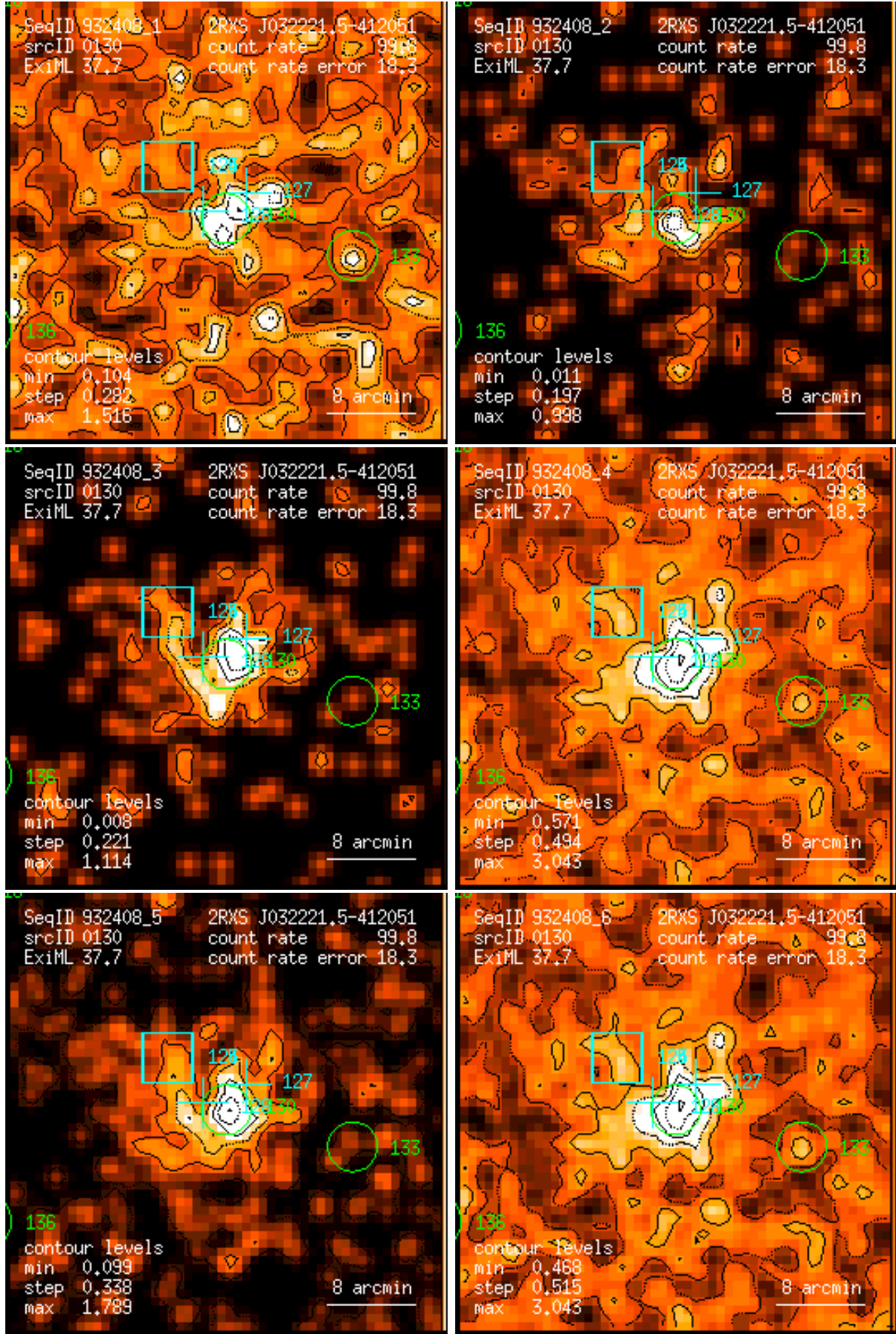
Figure 130: RASS 932408: detection 0130: band rate images, Gaussian filter: (1) PSPC channels 11 – 41, (2) 52 – 90, (3) 91 – 201, (4) 11 – 235, (5) 52 – 201, (6) 11 – 201. Broad band rates in counts/ks. Band rate contour levels in counts/ks/arcmin 2 .
