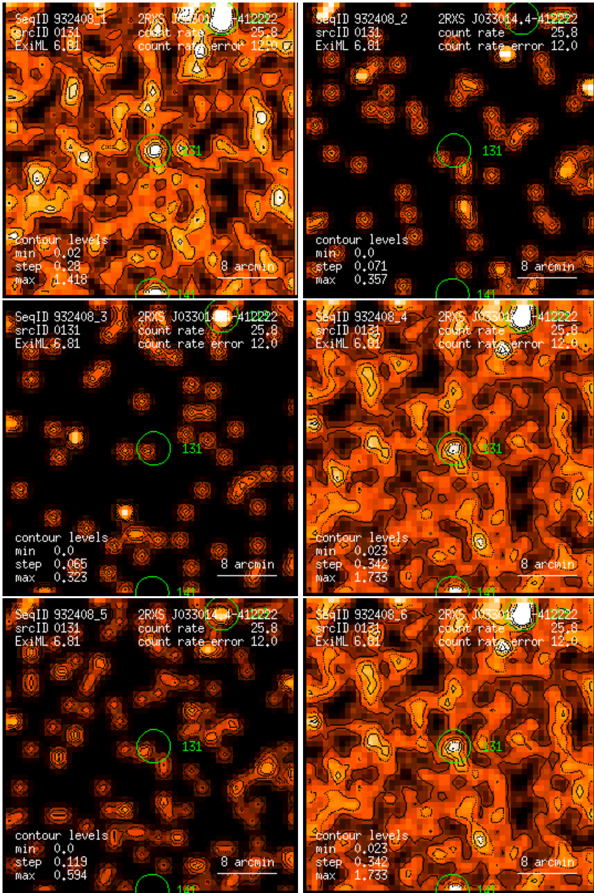
Figure 131: RASS 932408: detection 0131: band rate images, Gaussian filter: (1) PSPC channels 11 – 41, (2) 52 – 90, (3) 91 – 201, (4) 11 – 235, (5) 52 – 201, (6) 11 – 201. Broad band rates in counts/ks. Band rate contour levels in counts/ks/arcmin 2 .
