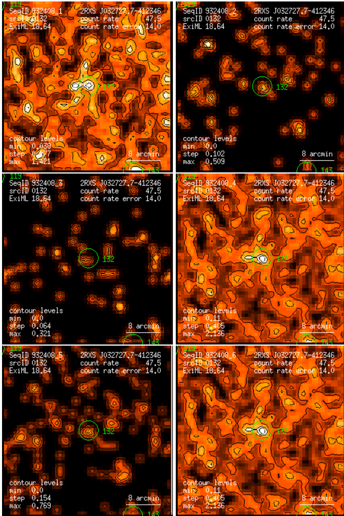
Figure 132: RASS 932408: detection 0132: band rate images, Gaussian filter: (1) PSPC channels 11 – 41, (2) 52 – 90, (3) 91 – 201, (4) 11 – 235, (5) 52 – 201, (6) 11 – 201. Broad band rates in counts/ks. Band rate contour levels in counts/ks/arcmin 2 .
