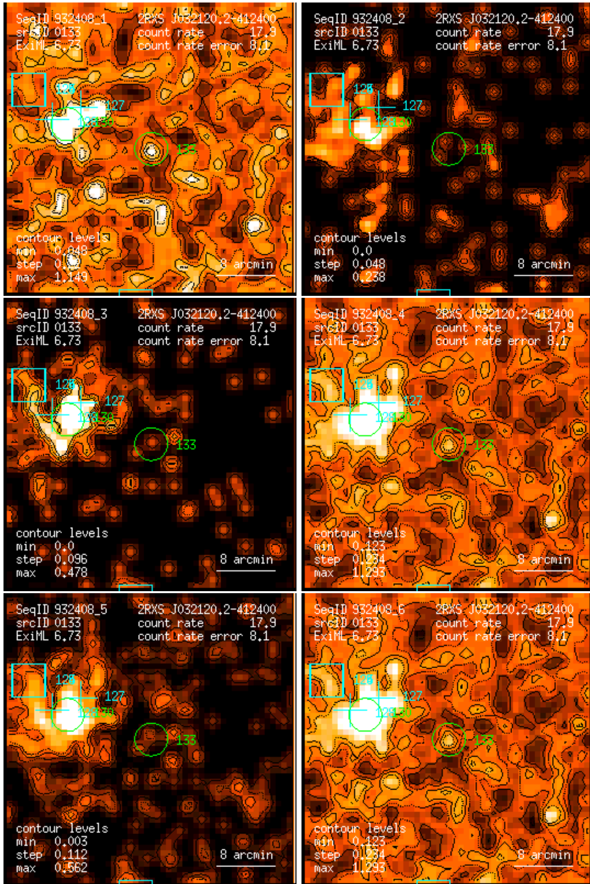
Figure 133: RASS 932408: detection 0133: band rate images, Gaussian filter: (1) PSPC channels 11 – 41, (2) 52 – 90, (3) 91 – 201, (4) 11 – 235, (5) 52 – 201, (6) 11 – 201. Broad band rates in counts/ks. Band rate contour levels in counts/ks/arcmin 2 .
