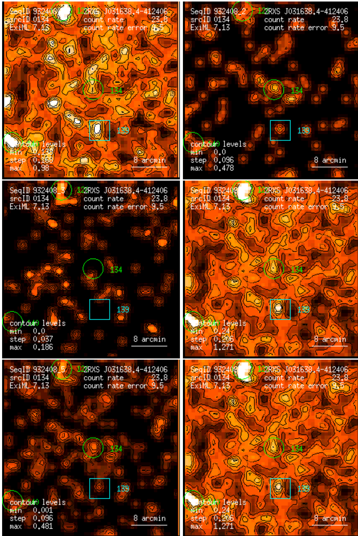
Figure 134: RASS 932408: detection 0134: band rate images, Gaussian filter: (1) PSPC channels 11 – 41, (2) 52 – 90, (3) 91 – 201, (4) 11 – 235, (5) 52 – 201, (6) 11 – 201. Broad band rates in counts/ks. Band rate contour levels in counts/ks/arcmin 2 .
