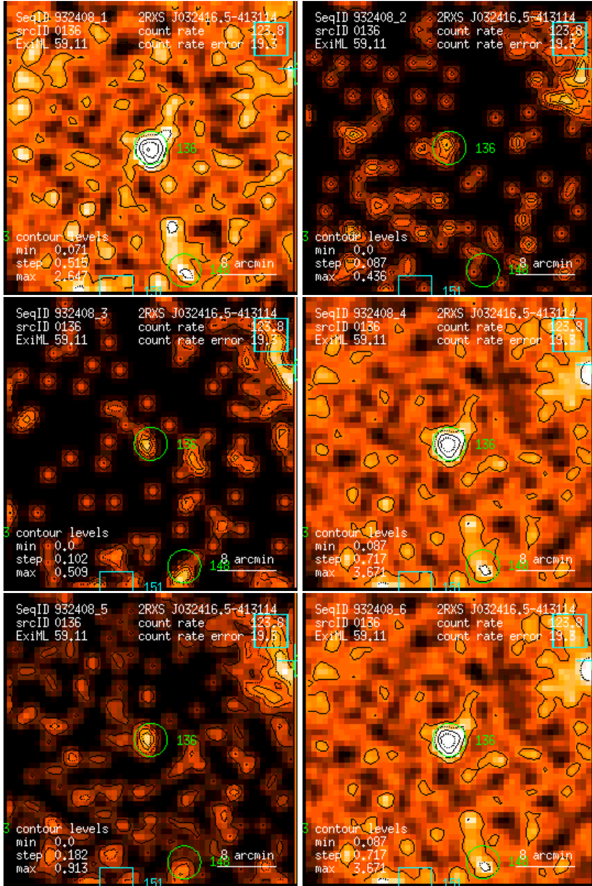
Figure 136: RASS 932408: detection 0136: band rate images, Gaussian filter: (1) PSPC channels 11 – 41, (2) 52 – 90, (3) 91 – 201, (4) 11 – 235, (5) 52 – 201, (6) 11 – 201. Broad band rates in counts/ks. Band rate contour levels in counts/ks/arcmin 2 .
