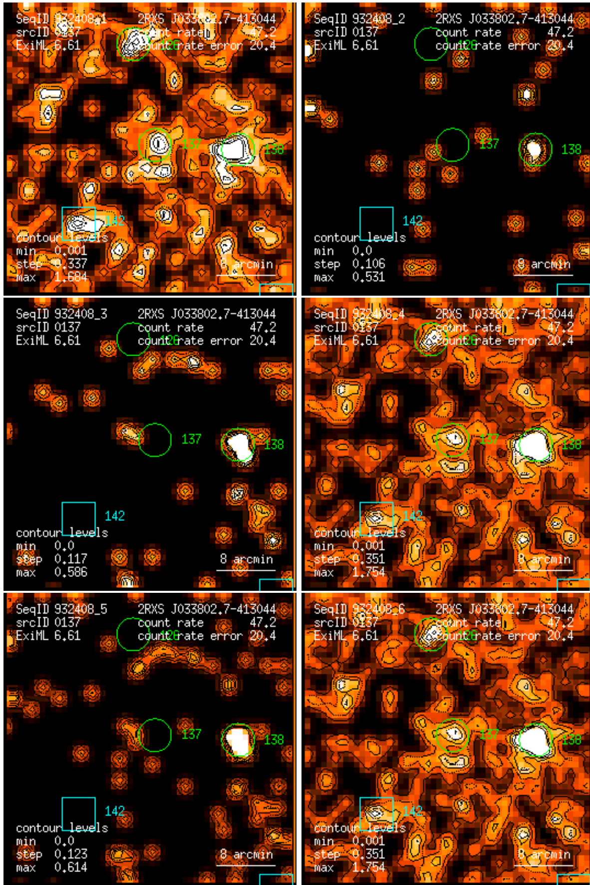
Figure 137: RASS 932408: detection 0137: band rate images, Gaussian filter: (1) PSPC channels 11 – 41, (2) 52 – 90, (3) 91 – 201, (4) 11 – 235, (5) 52 – 201, (6) 11 – 201. Broad band rates in counts/ks. Band rate contour levels in counts/ks/arcmin 2 .
