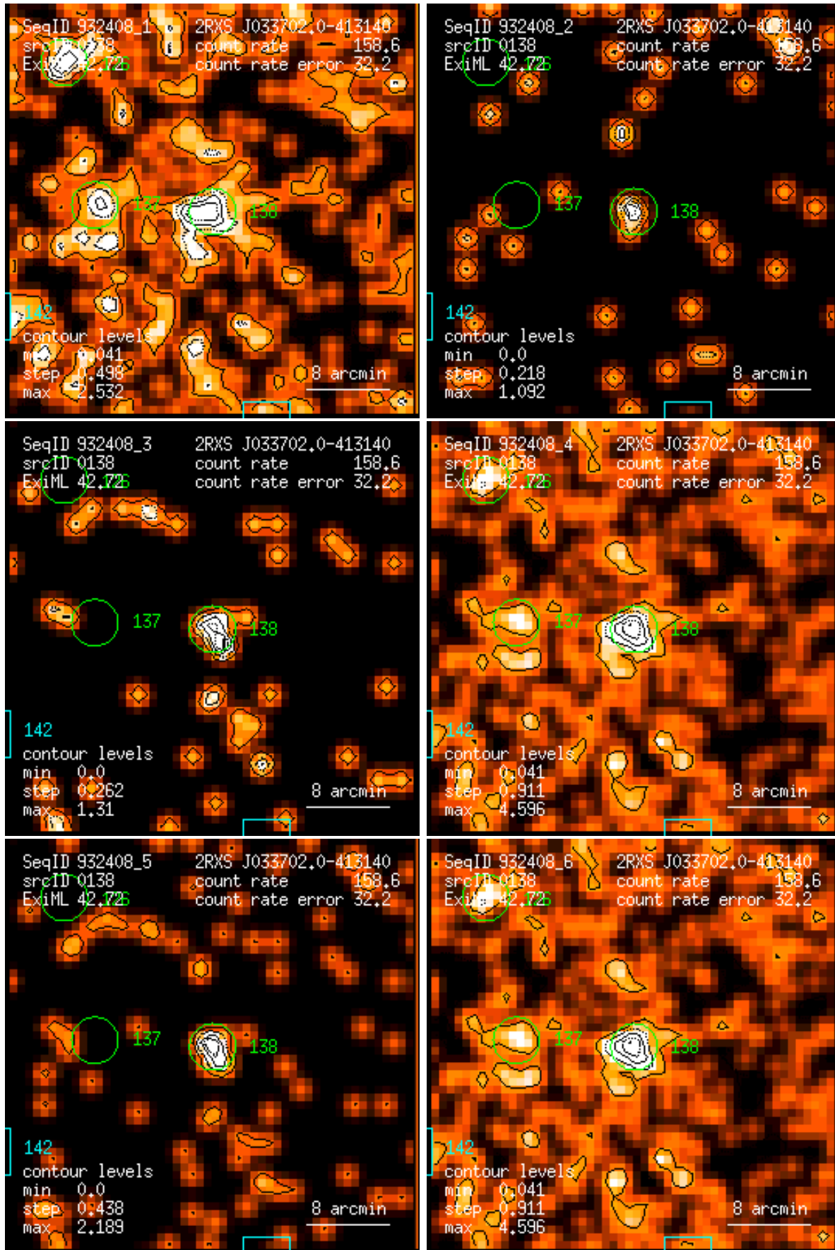
Figure 138: RASS 932408: detection 0138: band rate images, Gaussian filter: (1) PSPC channels 11 – 41, (2) 52 – 90, (3) 91 – 201, (4) 11 – 235, (5) 52 – 201, (6) 11 – 201. Broad band rates in counts/ks. Band rate contour levels in counts/ks/arcmin 2 .
