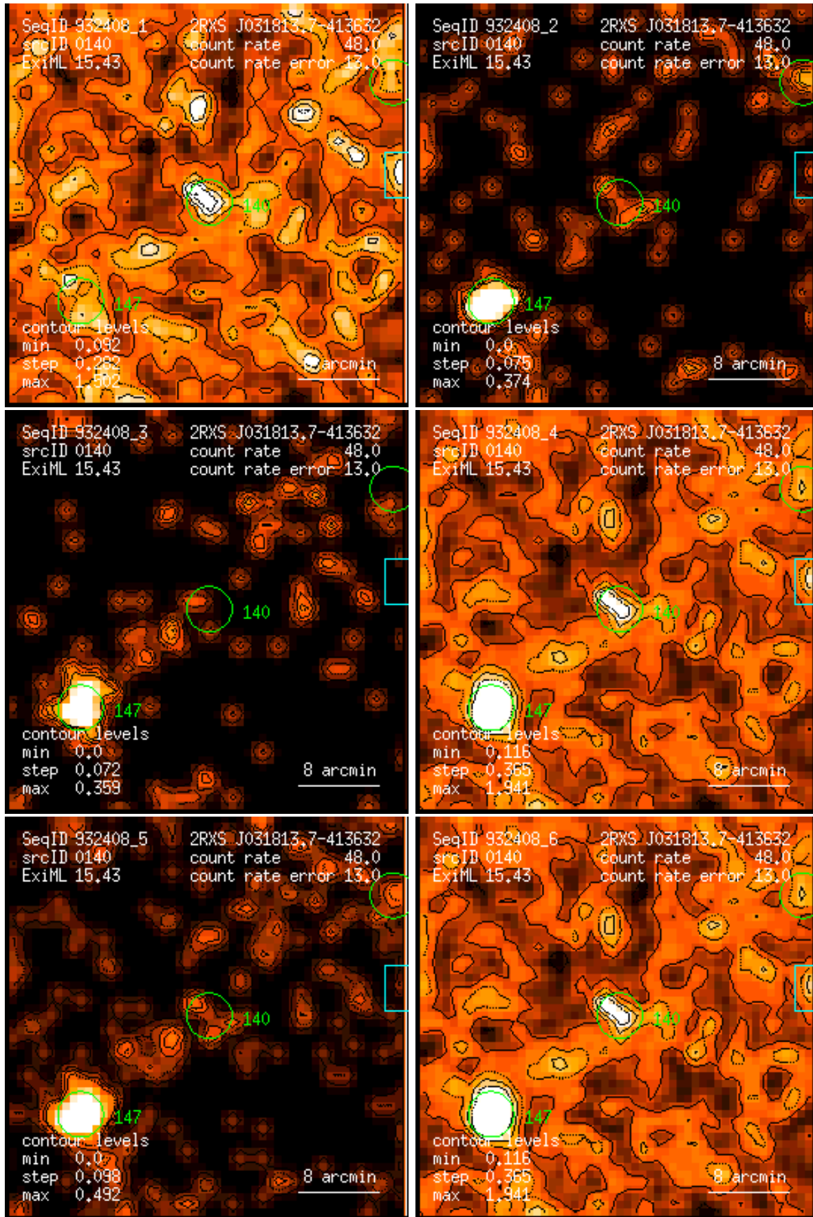
Figure 140: RASS 932408: detection 0140: band rate images, Gaussian filter: (1) PSPC channels 11 – 41, (2) 52 – 90, (3) 91 – 201, (4) 11 – 235, (5) 52 – 201, (6) 11 – 201. Broad band rates in counts/ks. Band rate contour levels in counts/ks/arcmin 2 .
