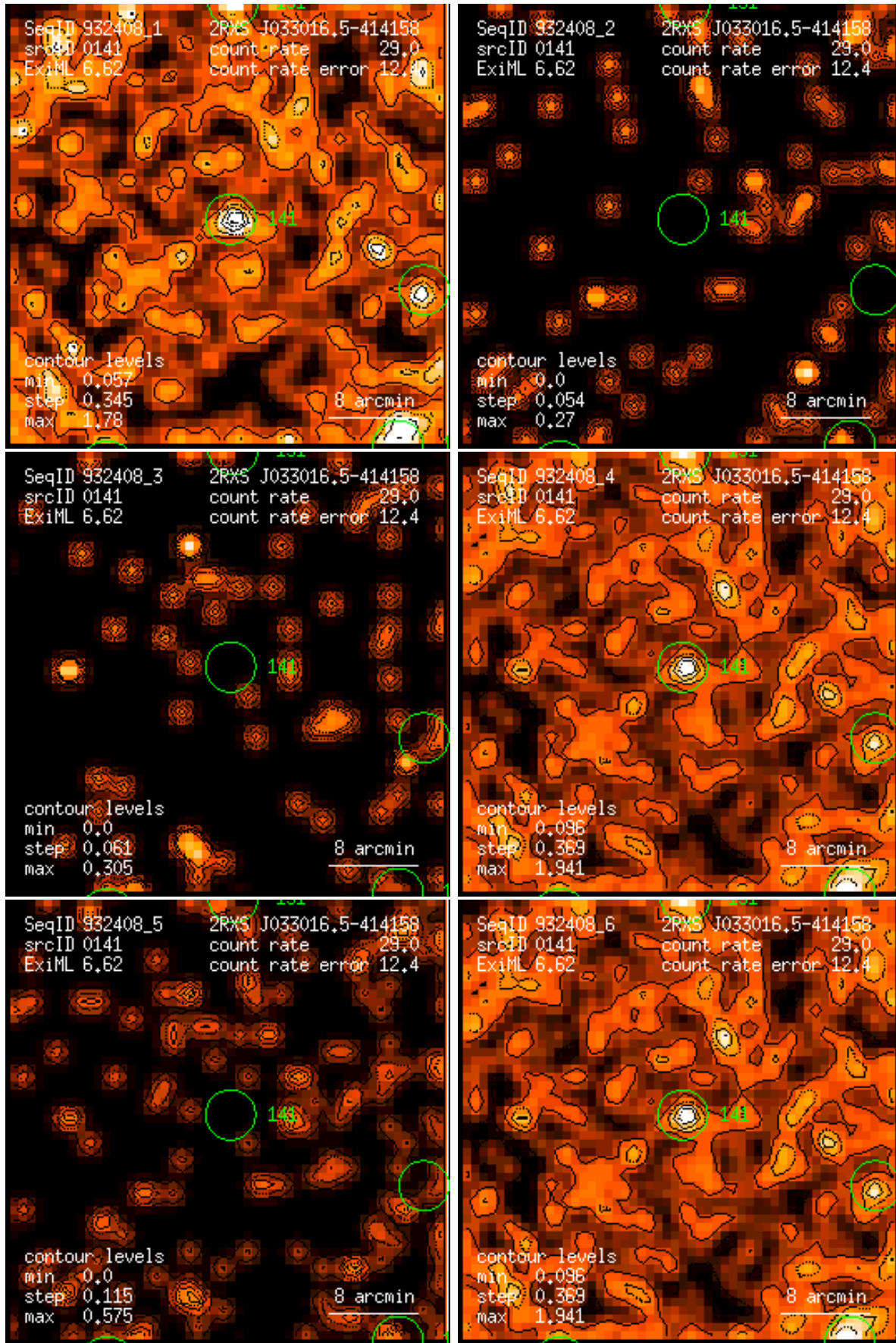
Figure 141: RASS 932408: detection 0141: band rate images, Gaussian filter: (1) PSPC channels 11 – 41, (2) 52 – 90, (3) 91 – 201, (4) 11 – 235, (5) 52 – 201, (6) 11 – 201. Broad band rates in counts/ks. Band rate contour levels in counts/ks/arcmin 2 .
