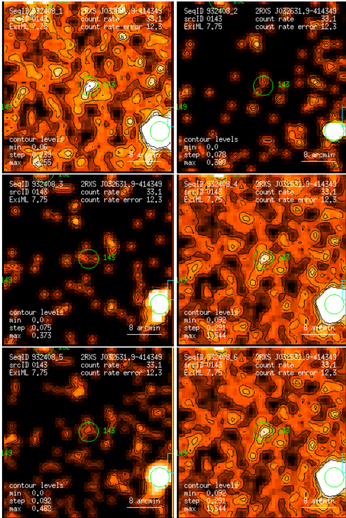
Figure 143: RASS 932408: detection 0143: band rate images, Gaussian filter: (1) PSPC channels 11 – 41, (2) 52 – 90, (3) 91 – 201, (4) 11 – 235, (5) 52 – 201, (6) 11 – 201. Broad band rates in counts/ks. Band rate contour levels in counts/ks/arcmin 2 .
