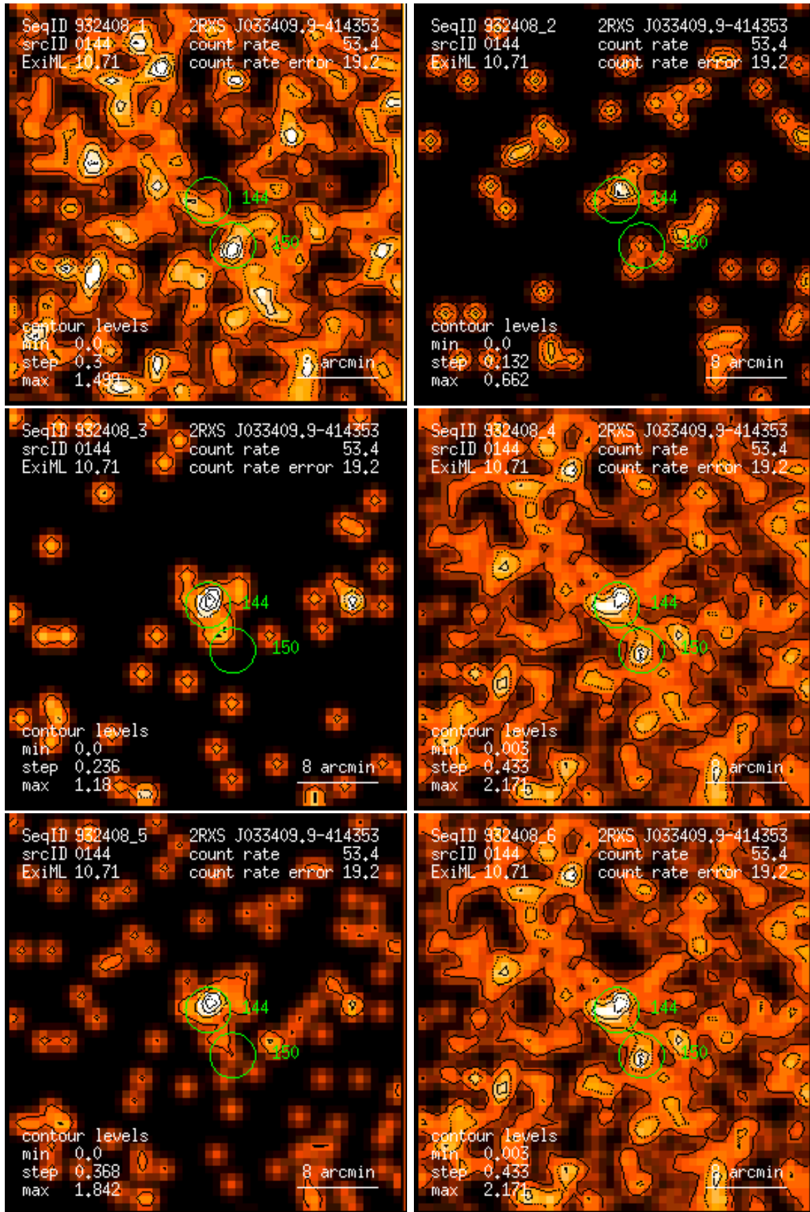
Figure 144: RASS 932408: detection 0144: band rate images, Gaussian filter: (1) PSPC channels 11 – 41, (2) 52 – 90, (3) 91 – 201, (4) 11 – 235, (5) 52 – 201, (6) 11 – 201. Broad band rates in counts/ks. Band rate contour levels in counts/ks/arcmin 2 .
