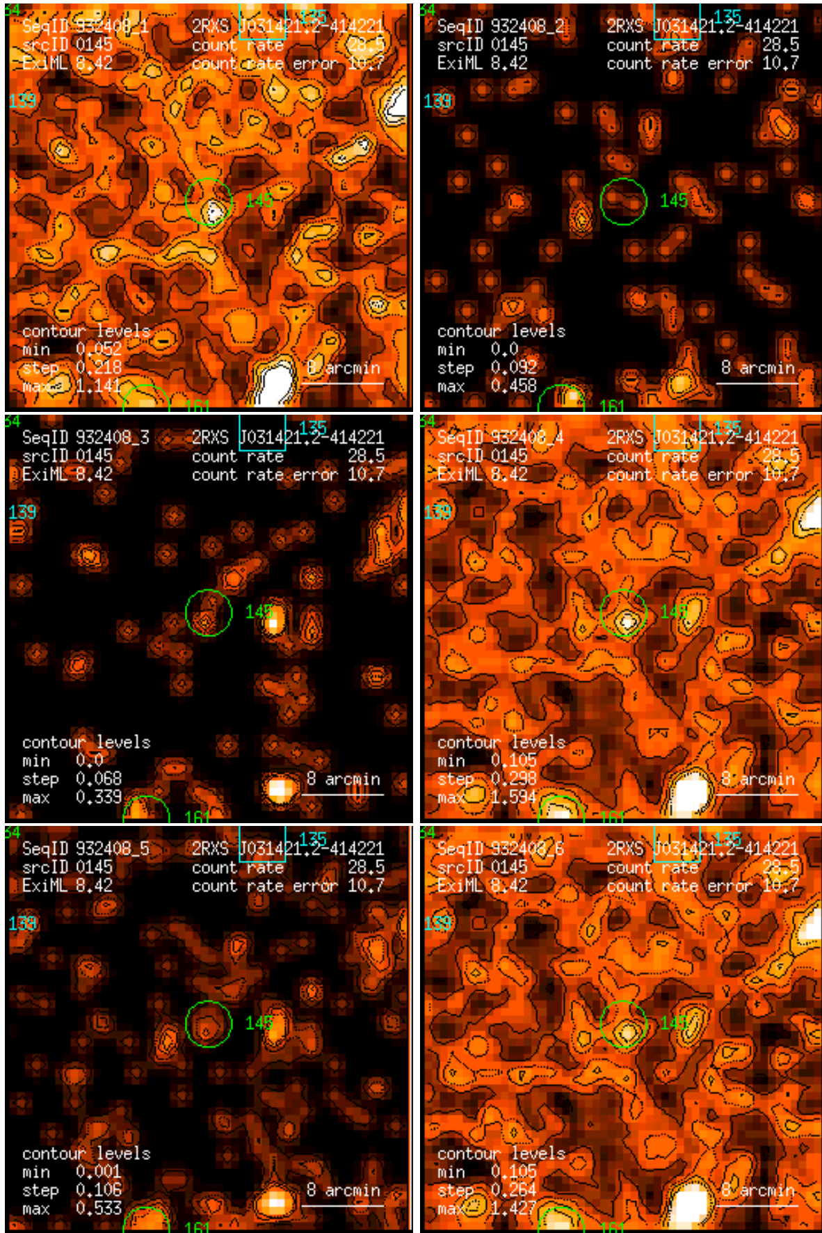
Figure 145: RASS 932408: detection 0145: band rate images, Gaussian filter: (1) PSPC channels 11 – 41, (2) 52 – 90, (3) 91 – 201, (4) 11 – 235, (5) 52 – 201, (6) 11 – 201. Broad band rates in counts/ks. Band rate contour levels in counts/ks/arcmin 2 .
