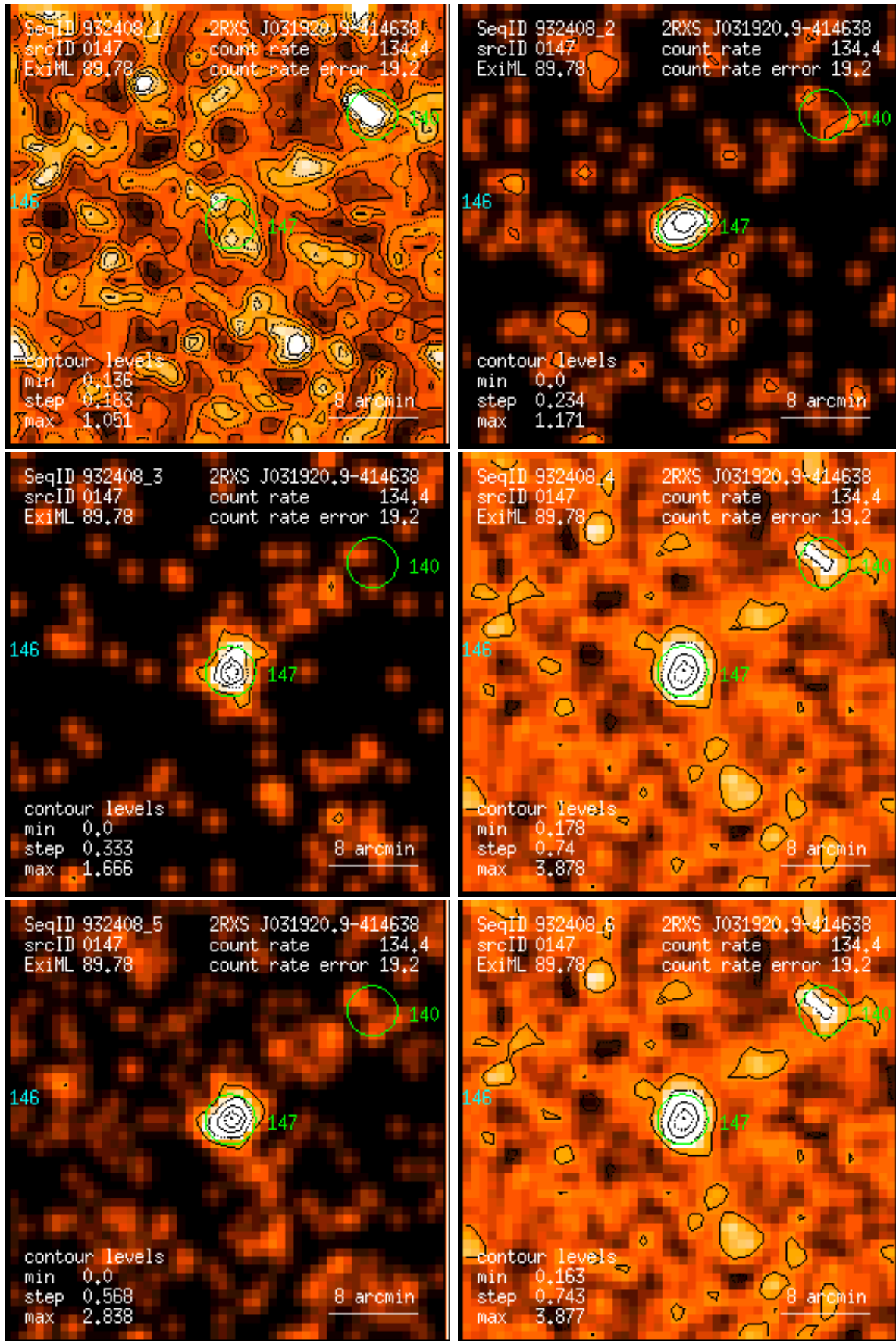
Figure 147: RASS 932408: detection 0147: band rate images, Gaussian filter: (1) PSPC channels 11 – 41, (2) 52 – 90, (3) 91 – 201, (4) 11 – 235, (5) 52 – 201, (6) 11 – 201. Broad band rates in counts/ks. Band rate contour levels in counts/ks/arcmin 2 .
