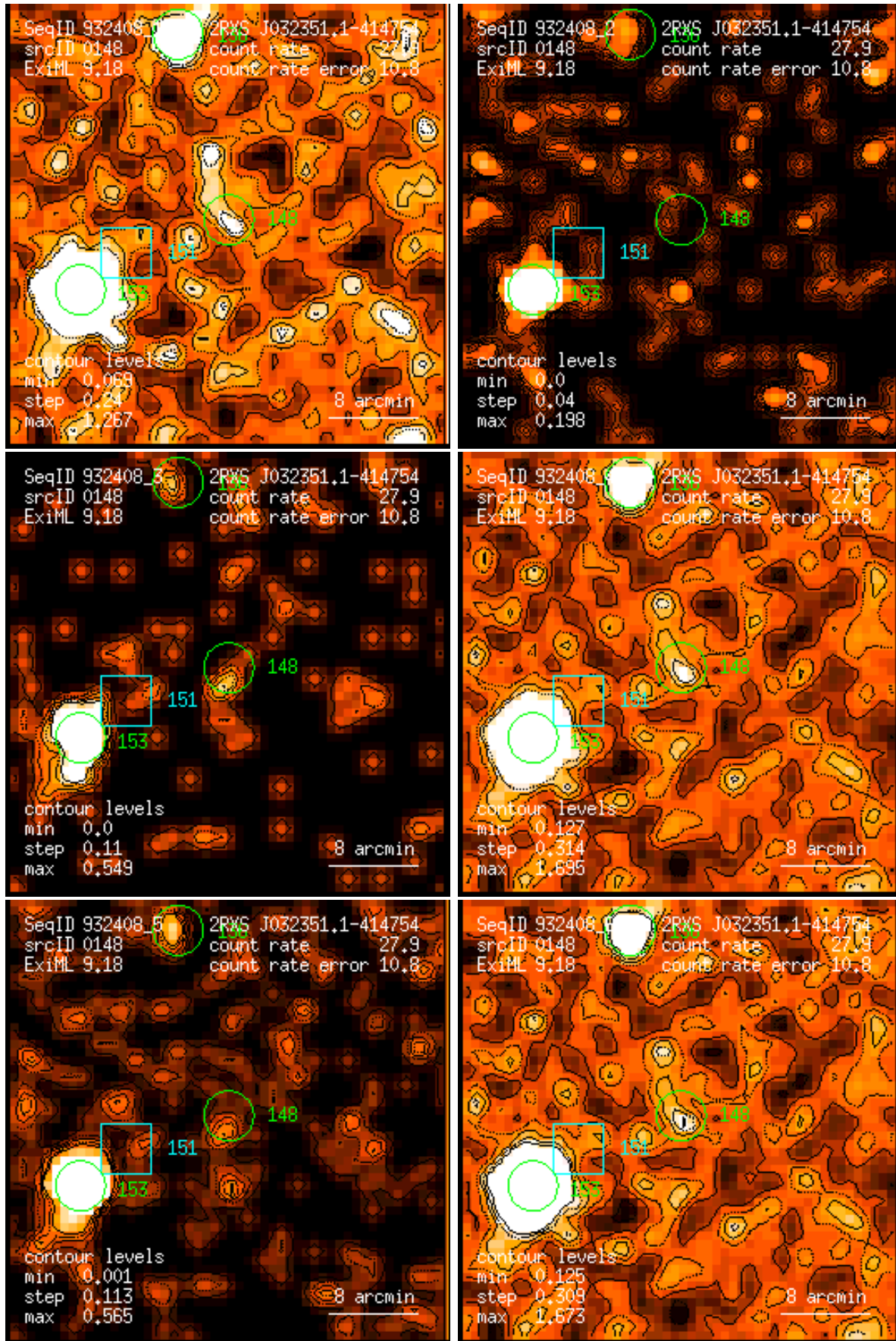
Figure 148: RASS 932408: detection 0148: band rate images, Gaussian filter: (1) PSPC channels 11 – 41, (2) 52 – 90, (3) 91 – 201, (4) 11 – 235, (5) 52 – 201, (6) 11 – 201. Broad band rates in counts/ks. Band rate contour levels in counts/ks/arcmin 2 .
