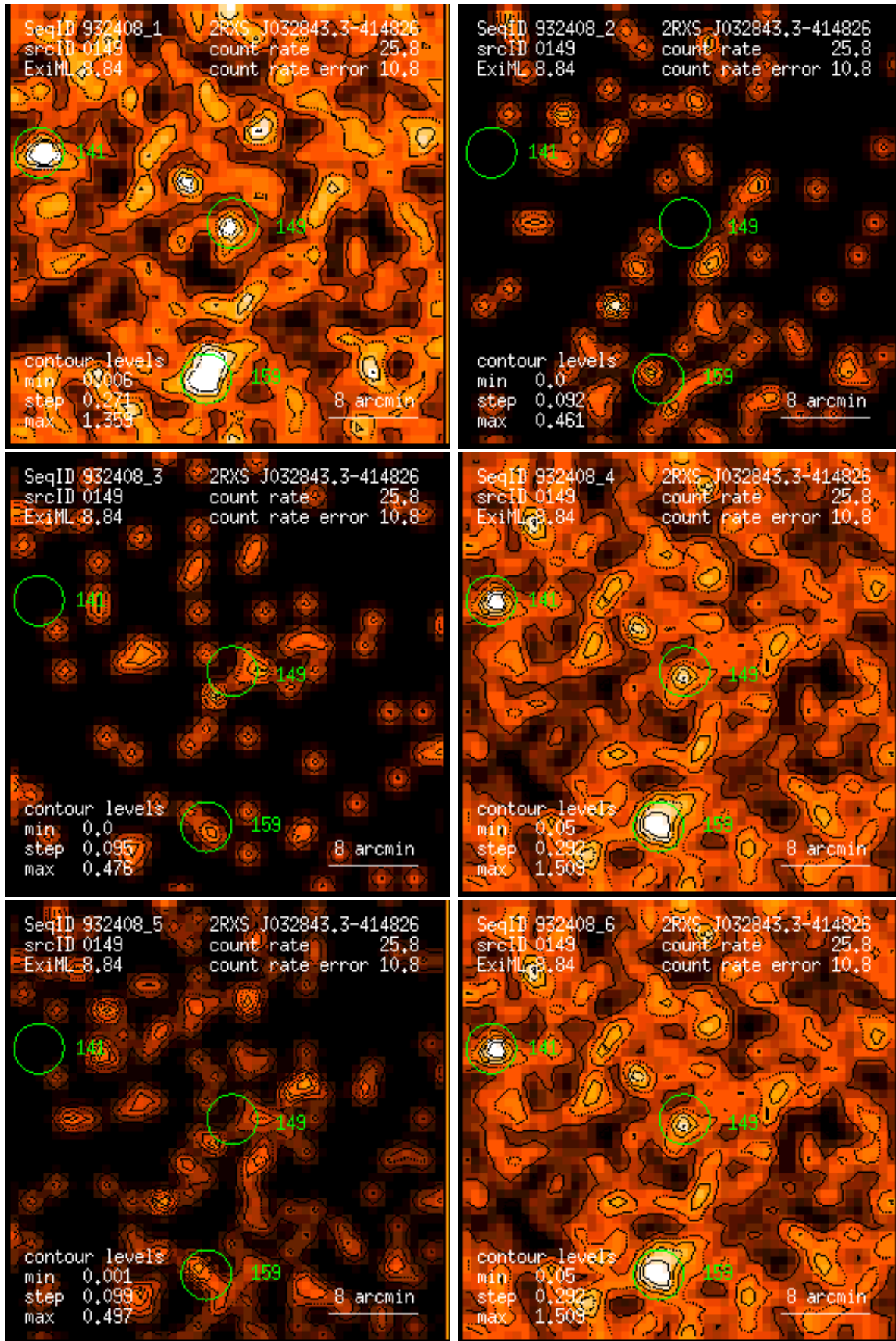
Figure 149: RASS 932408: detection 0149: band rate images, Gaussian filter: (1) PSPC channels 11 – 41, (2) 52 – 90, (3) 91 – 201, (4) 11 – 235, (5) 52 – 201, (6) 11 – 201. Broad band rates in counts/ks. Band rate contour levels in counts/ks/arcmin 2 .
