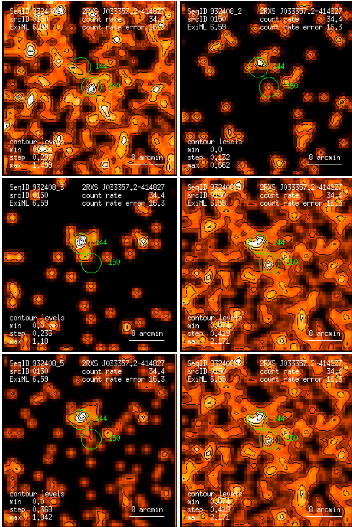
Figure 150: RASS 932408: detection 0150: band rate images, Gaussian filter: (1) PSPC channels 11 – 41, (2) 52 – 90, (3) 91 – 201, (4) 11 – 235, (5) 52 – 201, (6) 11 – 201. Broad band rates in counts/ks. Band rate contour levels in counts/ks/arcmin 2 .
