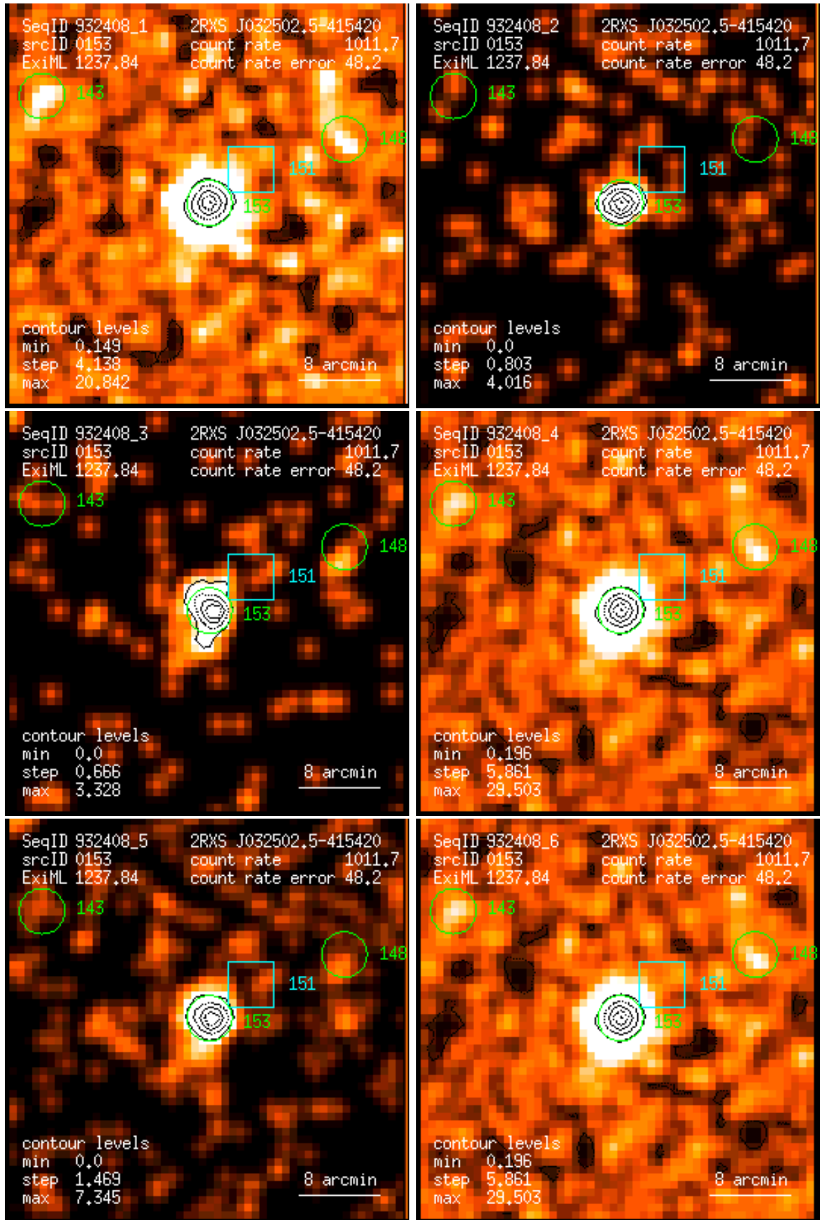
Figure 153: RASS 932408: detection 0153: band rate images, Gaussian filter: (1) PSPC channels 11 – 41, (2) 52 – 90, (3) 91 – 201, (4) 11 – 235, (5) 52 – 201, (6) 11 – 201. Broad band rates in counts/ks. Band rate contour levels in counts/ks/arcmin 2 .
