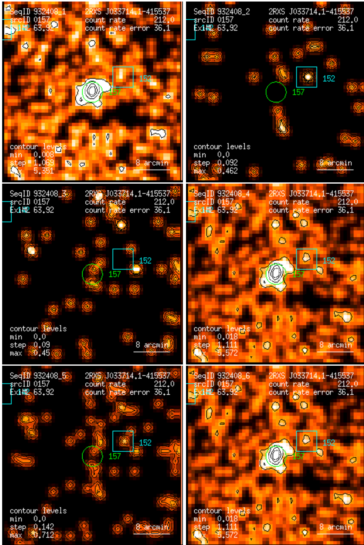
Figure 157: RASS 932408: detection 0157: band rate images, Gaussian filter: (1) PSPC channels 11 – 41, (2) 52 – 90, (3) 91 – 201, (4) 11 – 235, (5) 52 – 201, (6) 11 – 201. Broad band rates in counts/ks. Band rate contour levels in counts/ks/arcmin 2 .
