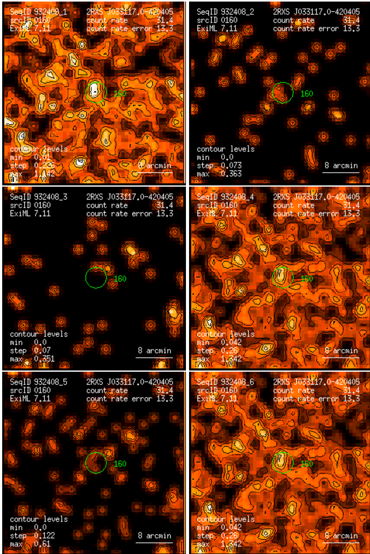
Figure 160: RASS 932408: detection 0160: band rate images, Gaussian filter: (1) PSPC channels 11 – 41, (2) 52 – 90, (3) 91 – 201, (4) 11 – 235, (5) 52 – 201, (6) 11 – 201. Broad band rates in counts/ks. Band rate contour levels in counts/ks/arcmin 2 .
