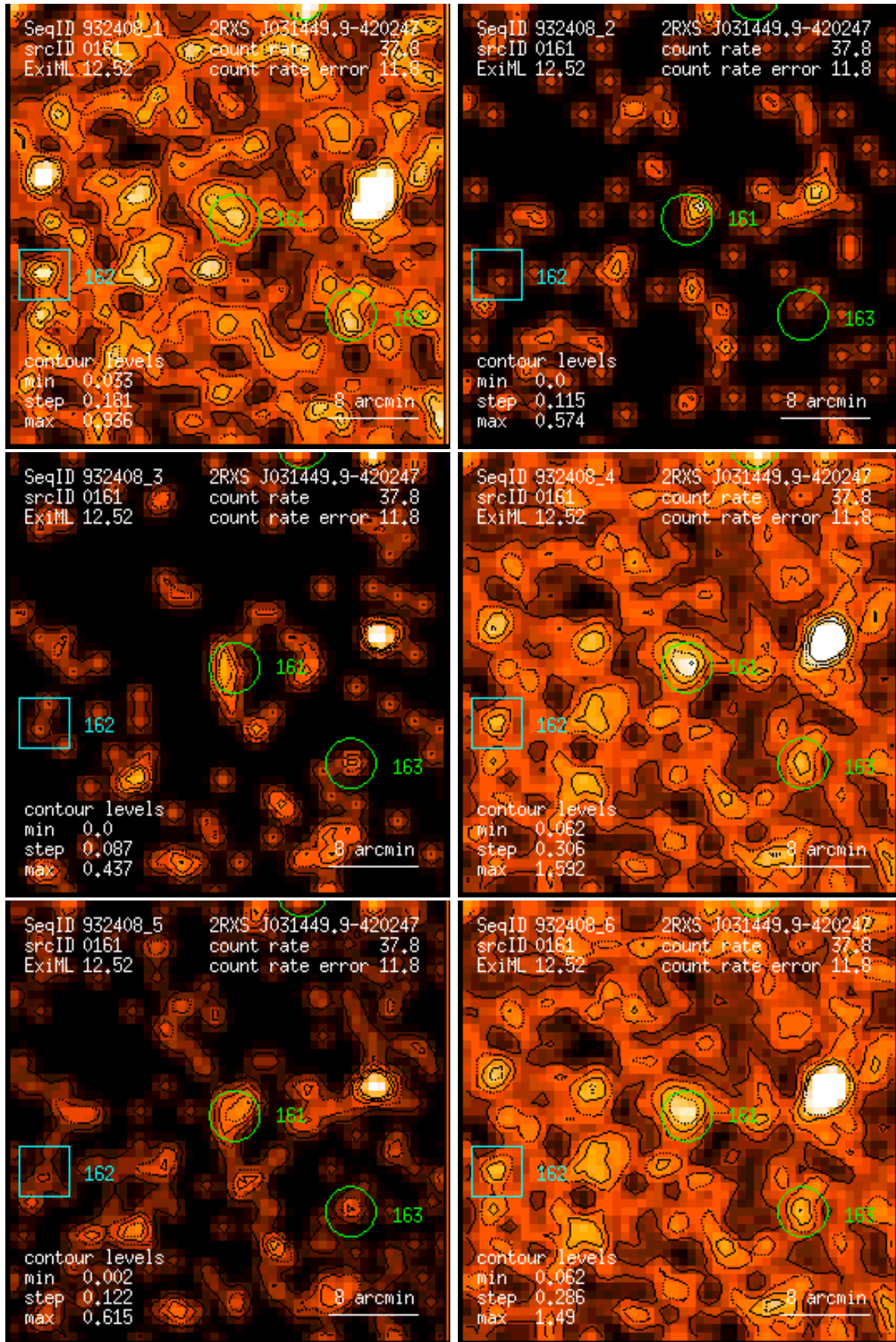
Figure 161: RASS 932408: detection 0161: band rate images, Gaussian filter: (1) PSPC channels 11 – 41, (2) 52 – 90, (3) 91 – 201, (4) 11 – 235, (5) 52 – 201, (6) 11 – 201. Broad band rates in counts/ks. Band rate contour levels in counts/ks/arcmin 2 .
