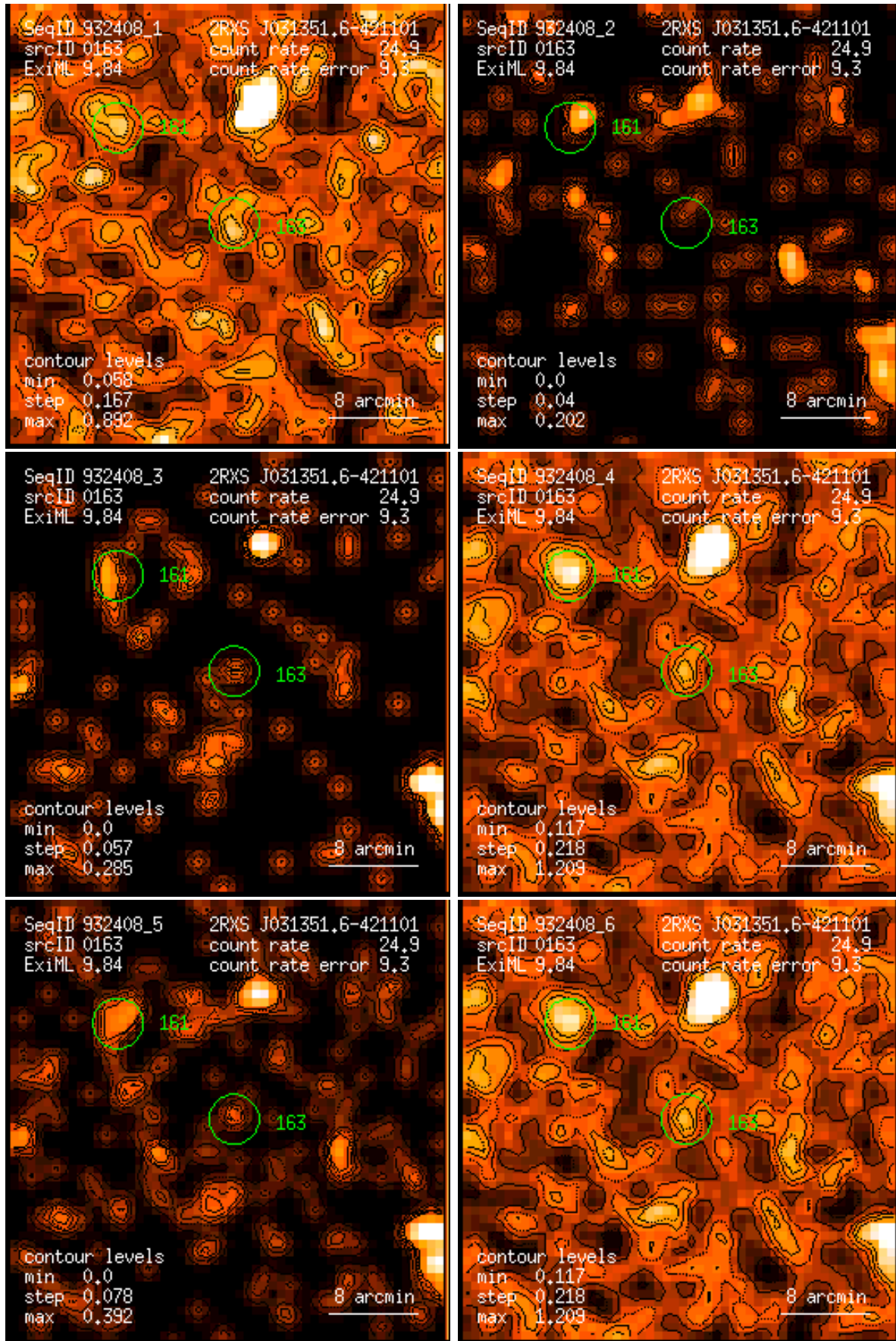
Figure 163: RASS 932408: detection 0163: band rate images, Gaussian filter: (1) PSPC channels 11 – 41, (2) 52 – 90, (3) 91 – 201, (4) 11 – 235, (5) 52 – 201, (6) 11 – 201. Broad band rates in counts/ks. Band rate contour levels in counts/ks/arcmin 2 .
